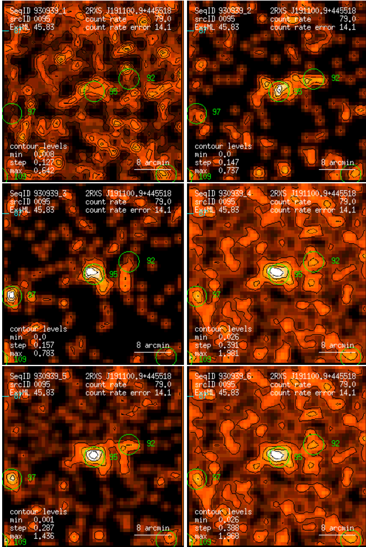
Figure 95: RASS 930939: detection 0095: band rate images, Gaussian filter: (1) PSPC channels 11 – 41, (2) 52 – 90, (3) 91 – 201, (4) 11 – 235, (5) 52 – 201, (6) 11 – 201. Broad band rates in counts/ks. Band rate contour levels in counts/ks/arcmin 2 .
