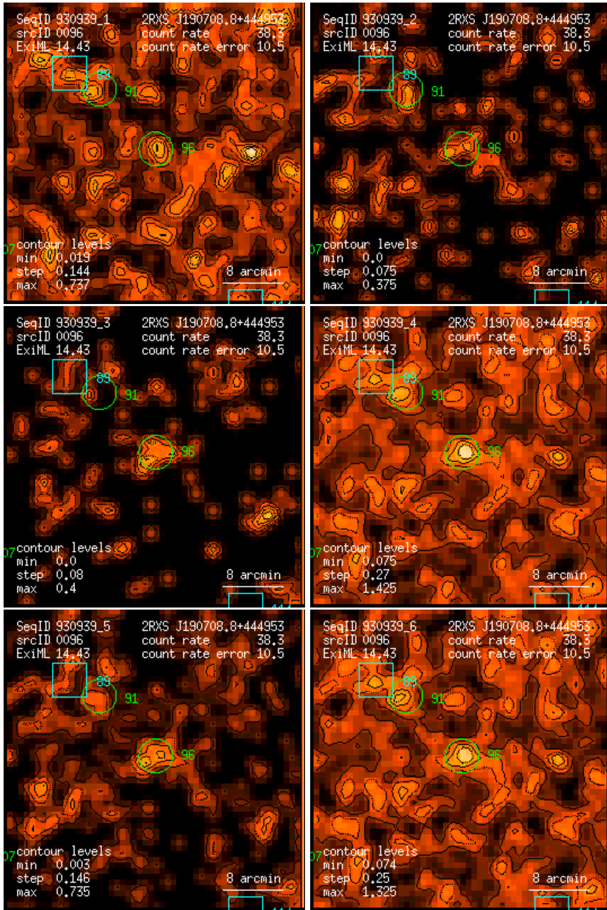
Figure 96: RASS 930939: detection 0096: band rate images, Gaussian filter: (1) PSPC channels 11 – 41, (2) 52 – 90, (3) 91 – 201, (4) 11 – 235, (5) 52 – 201, (6) 11 – 201. Broad band rates in counts/ks. Band rate contour levels in counts/ks/arcmin 2 .
