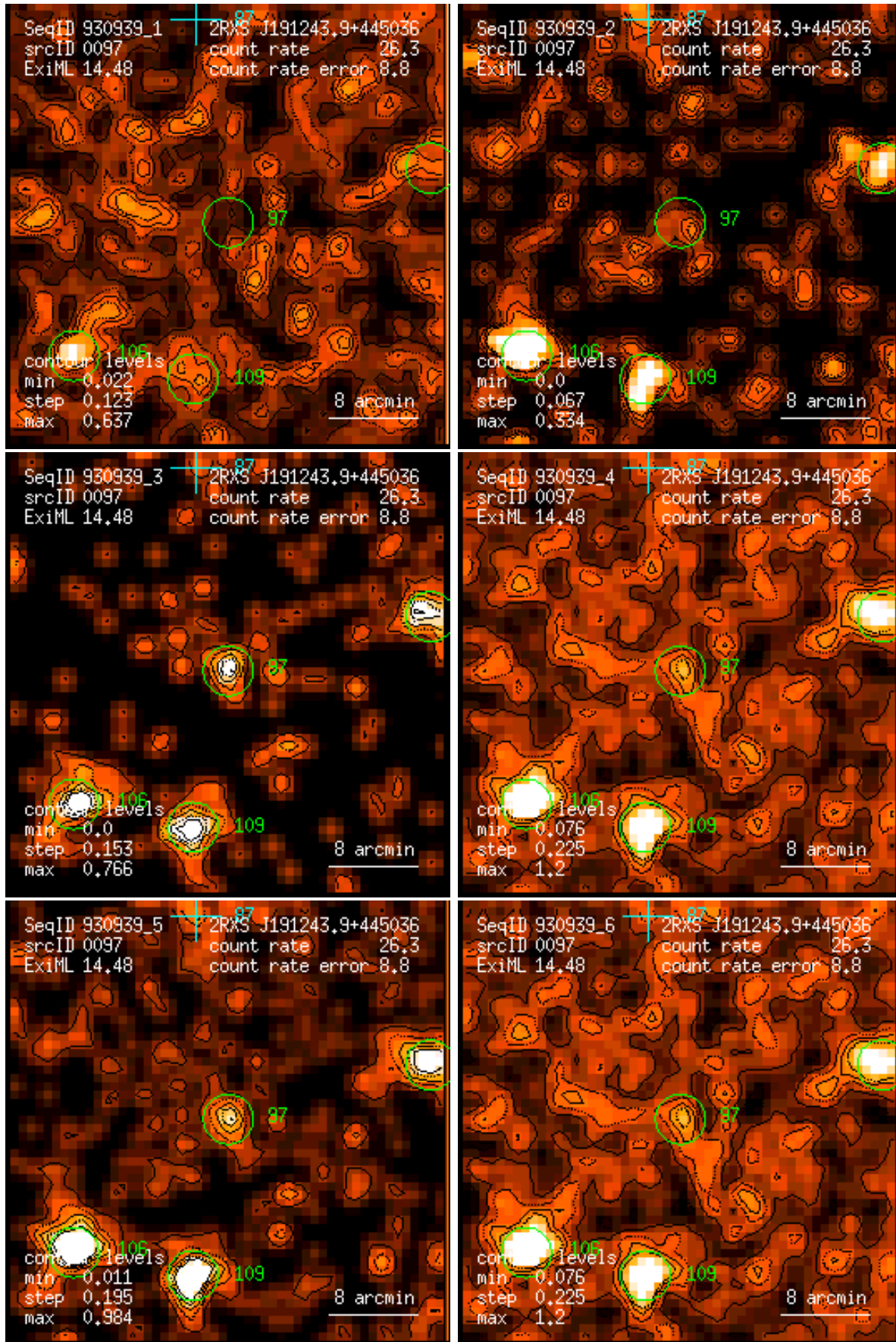
Figure 97: RASS 930939: detection 0097: band rate images, Gaussian filter: (1) PSPC channels 11 – 41, (2) 52 – 90, (3) 91 – 201, (4) 11 – 235, (5) 52 – 201, (6) 11 – 201. Broad band rates in counts/ks. Band rate contour levels in counts/ks/arcmin 2 .
