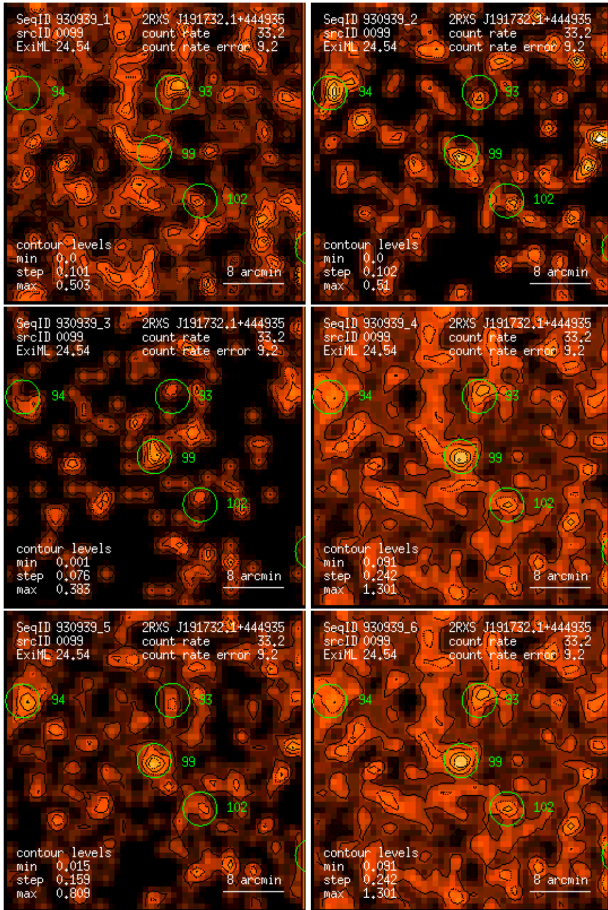
Figure 99: RASS 930939: detection 0099: band rate images, Gaussian filter: (1) PSPC channels 11 – 41, (2) 52 – 90, (3) 91 – 201, (4) 11 – 235, (5) 52 – 201, (6) 11 – 201. Broad band rates in counts/ks. Band rate contour levels in counts/ks/arcmin 2 .
