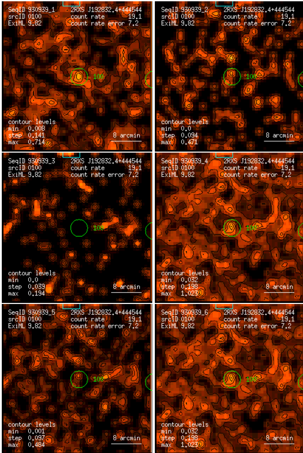
Figure 100: RASS 930939: detection 0100: band rate images, Gaussian filter: (1) PSPC channels 11 – 41, (2) 52 – 90, (3) 91 – 201, (4) 11 – 235, (5) 52 – 201, (6) 11 – 201. Broad band rates in counts/ks. Band rate contour levels in counts/ks/arcmin 2 .
