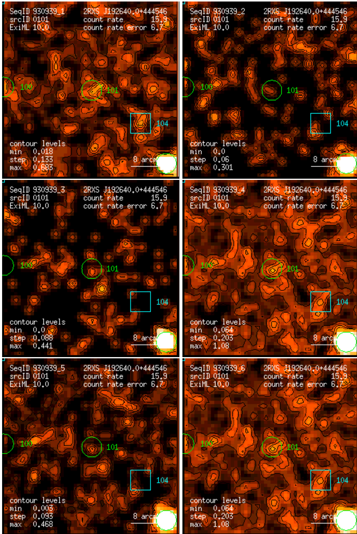
Figure 101: RASS 930939: detection 0101: band rate images, Gaussian filter: (1) PSPC channels 11 – 41, (2) 52 – 90, (3) 91 – 201, (4) 11 – 235, (5) 52 – 201, (6) 11 – 201. Broad band rates in counts/ks. Band rate contour levels in counts/ks/arcmin 2 .
