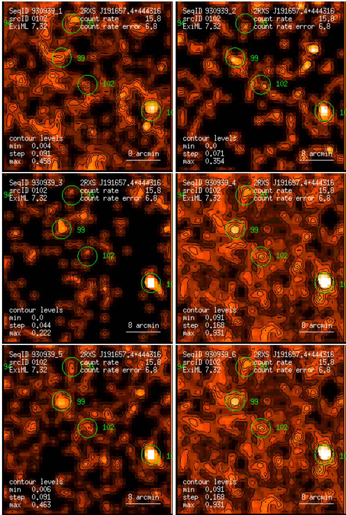
Figure 102: RASS 930939: detection 0102: band rate images, Gaussian filter: (1) PSPC channels 11 – 41, (2) 52 – 90, (3) 91 – 201, (4) 11 – 235, (5) 52 – 201, (6) 11 – 201. Broad band rates in counts/ks. Band rate contour levels in counts/ks/arcmin 2 .
