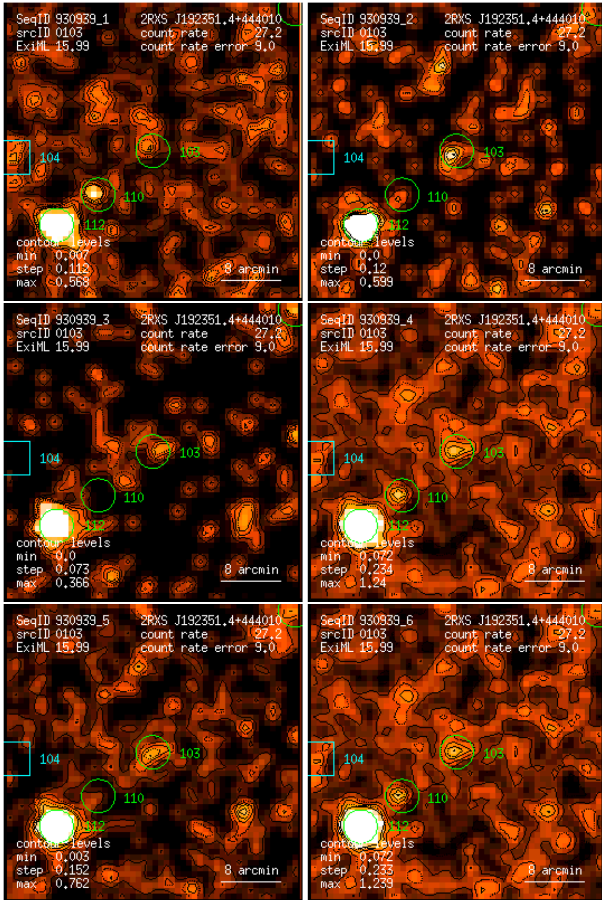
Figure 103: RASS 930939: detection 0103: band rate images, Gaussian filter: (1) PSPC channels 11 – 41, (2) 52 – 90, (3) 91 – 201, (4) 11 – 235, (5) 52 – 201, (6) 11 – 201. Broad band rates in counts/ks. Band rate contour levels in counts/ks/arcmin 2 .
