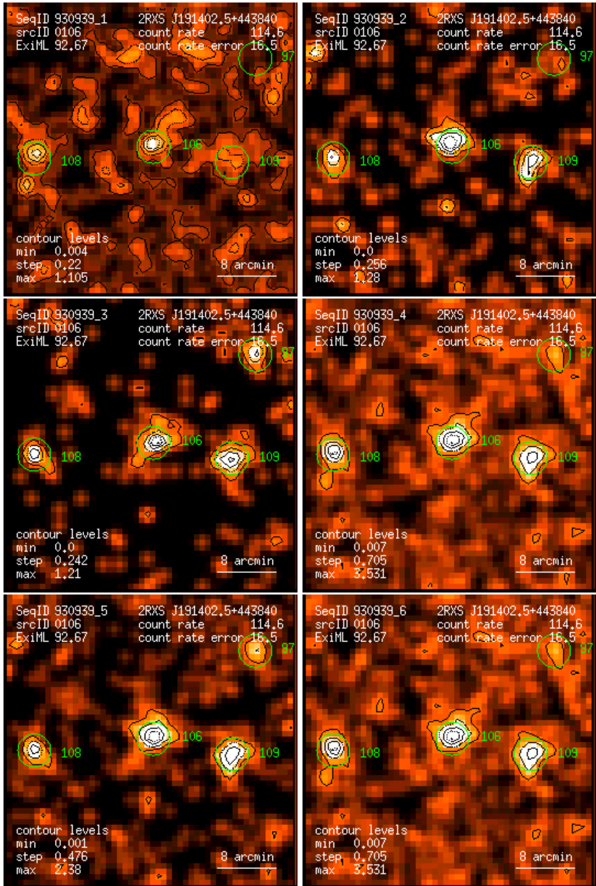
Figure 106: RASS 930939: detection 0106: band rate images, Gaussian filter: (1) PSPC channels 11 – 41, (2) 52 – 90, (3) 91 – 201, (4) 11 – 235, (5) 52 – 201, (6) 11 – 201. Broad band rates in counts/ks. Band rate contour levels in counts/ks/arcmin 2 .
