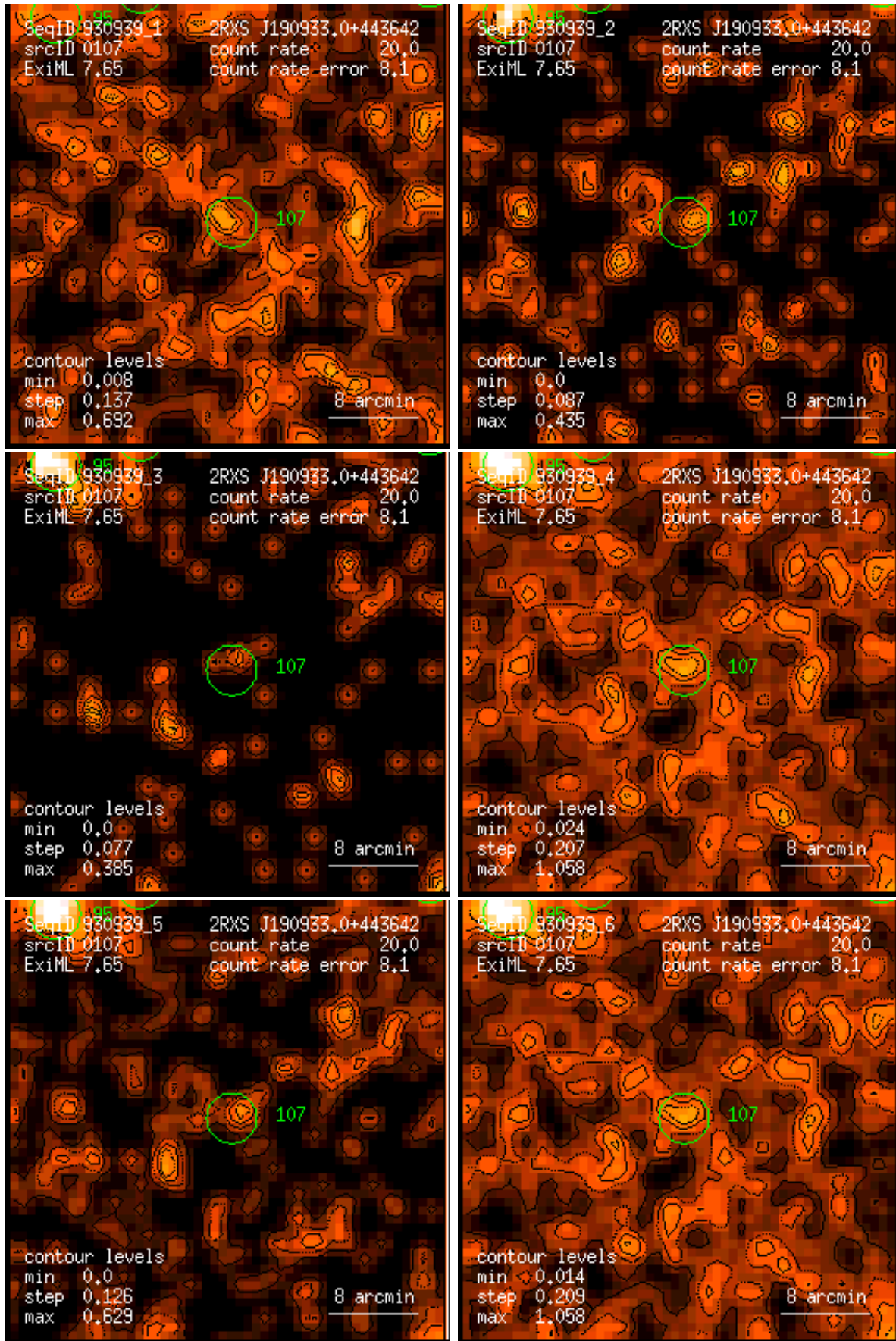
Figure 107: RASS 930939: detection 0107: band rate images, Gaussian filter: (1) PSPC channels 11 – 41, (2) 52 – 90, (3) 91 – 201, (4) 11 – 235, (5) 52 – 201, (6) 11 – 201. Broad band rates in counts/ks. Band rate contour levels in counts/ks/arcmin 2 .
