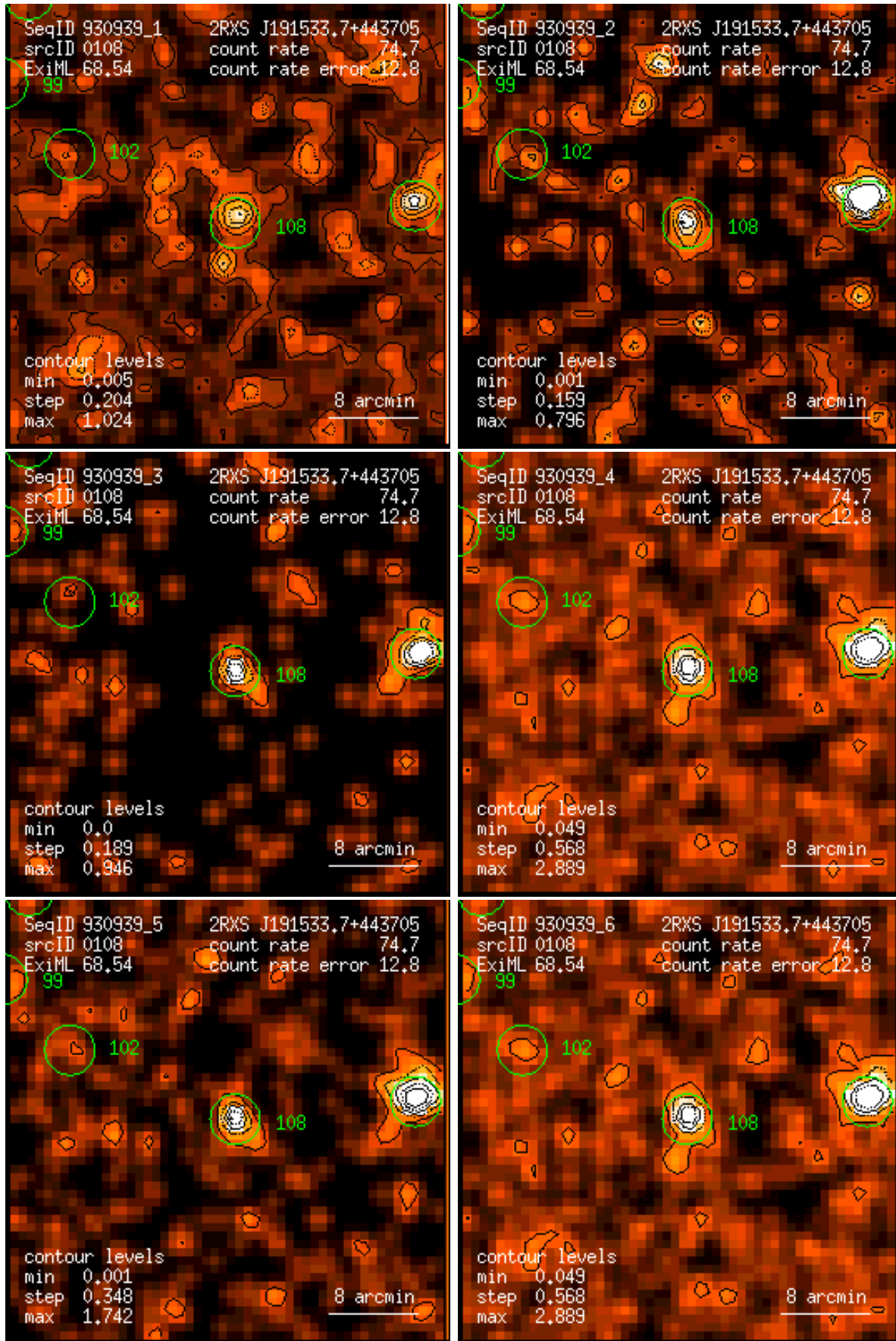
Figure 108: RASS 930939: detection 0108: band rate images, Gaussian filter: (1) PSPC channels 11 – 41, (2) 52 – 90, (3) 91 – 201, (4) 11 – 235, (5) 52 – 201, (6) 11 – 201. Broad band rates in counts/ks. Band rate contour levels in counts/ks/arcmin 2 .
