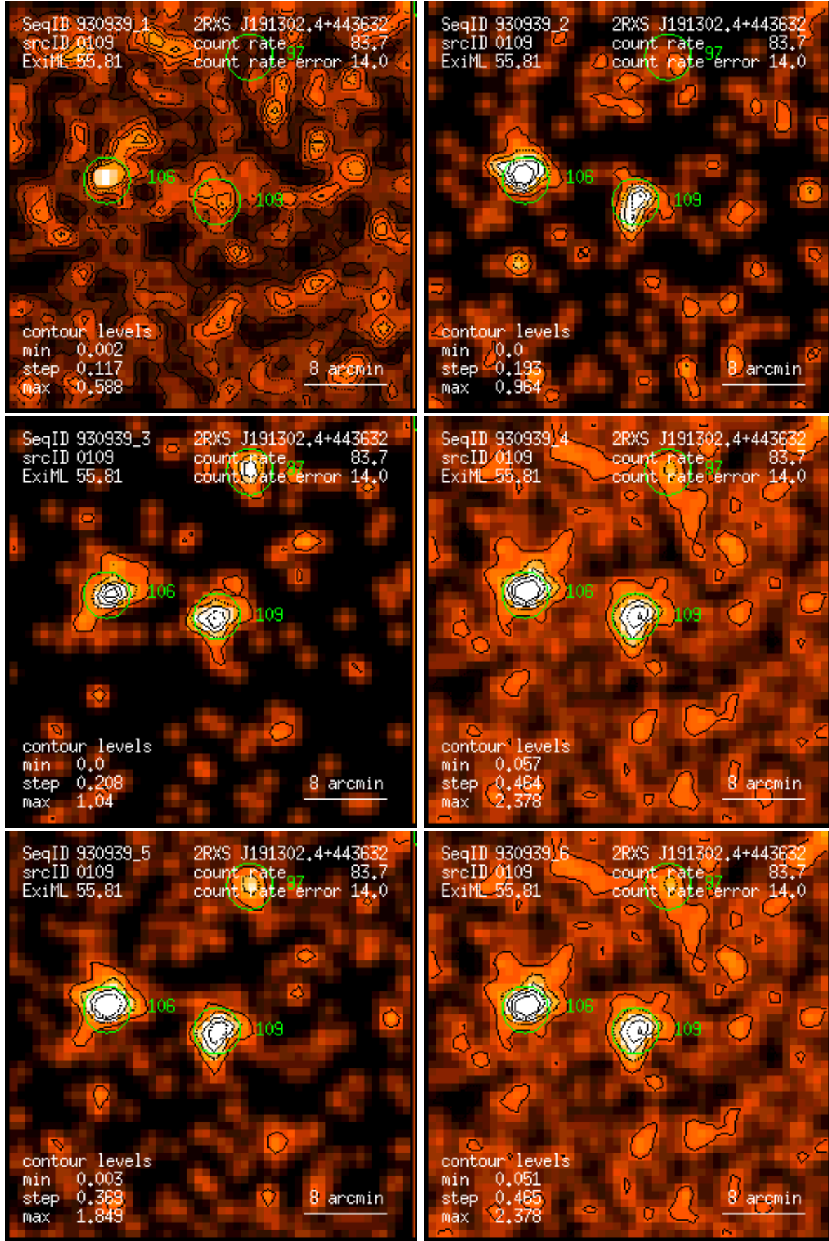
Figure 109: RASS 930939: detection 0109: band rate images, Gaussian filter: (1) PSPC channels 11 – 41, (2) 52 – 90, (3) 91 – 201, (4) 11 – 235, (5) 52 – 201, (6) 11 – 201. Broad band rates in counts/ks. Band rate contour levels in counts/ks/arcmin 2 .
