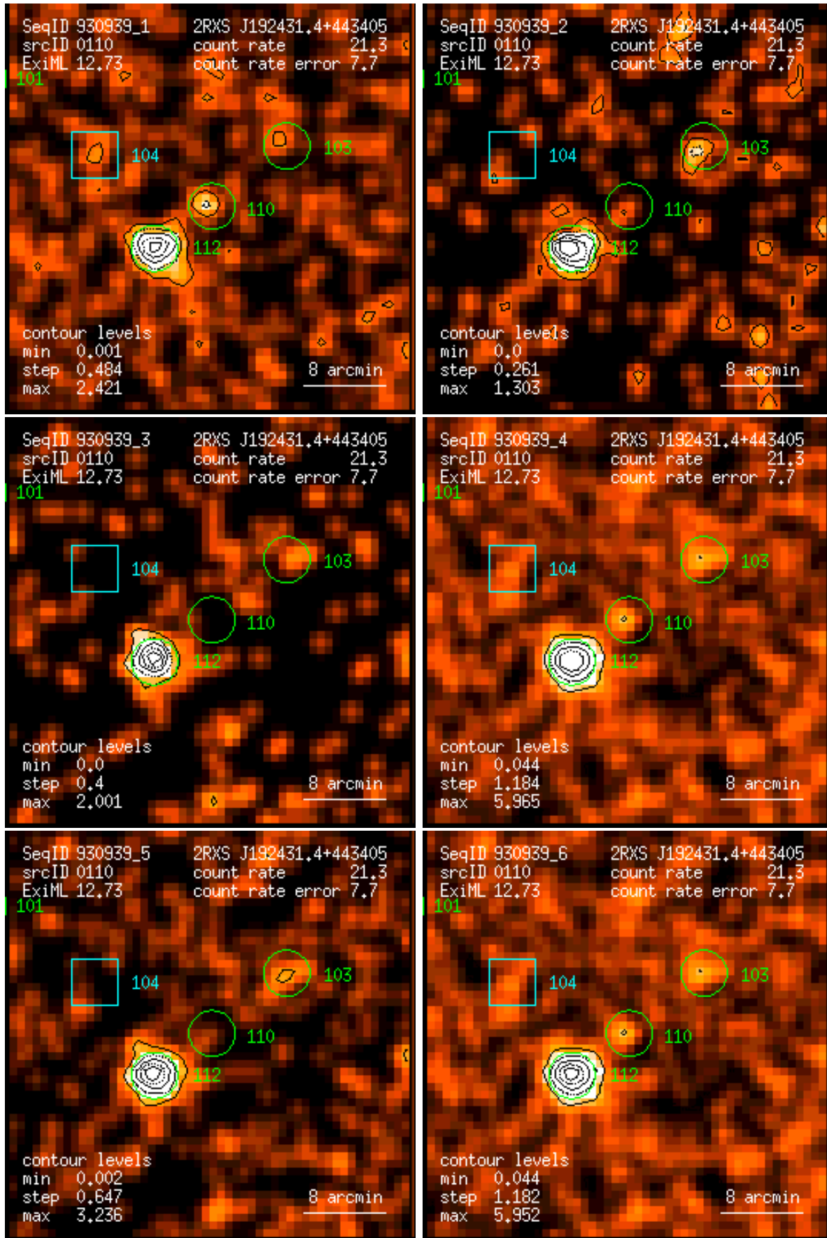
Figure 110: RASS 930939: detection 0110: band rate images, Gaussian filter: (1) PSPC channels 11 – 41, (2) 52 – 90, (3) 91 – 201, (4) 11 – 235, (5) 52 – 201, (6) 11 – 201. Broad band rates in counts/ks. Band rate contour levels in counts/ks/arcmin 2 .
