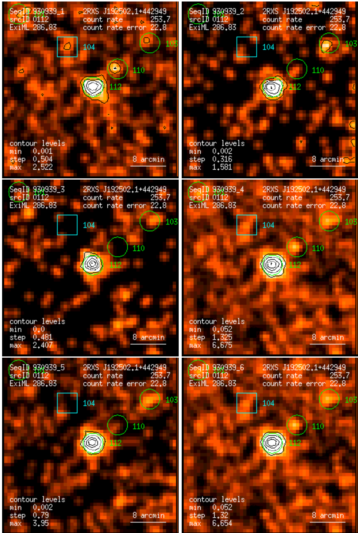
Figure 112: RASS 930939: detection 0112: band rate images, Gaussian filter: (1) PSPC channels 11 – 41, (2) 52 – 90, (3) 91 – 201, (4) 11 – 235, (5) 52 – 201, (6) 11 – 201. Broad band rates in counts/ks. Band rate contour levels in counts/ks/arcmin 2 .
