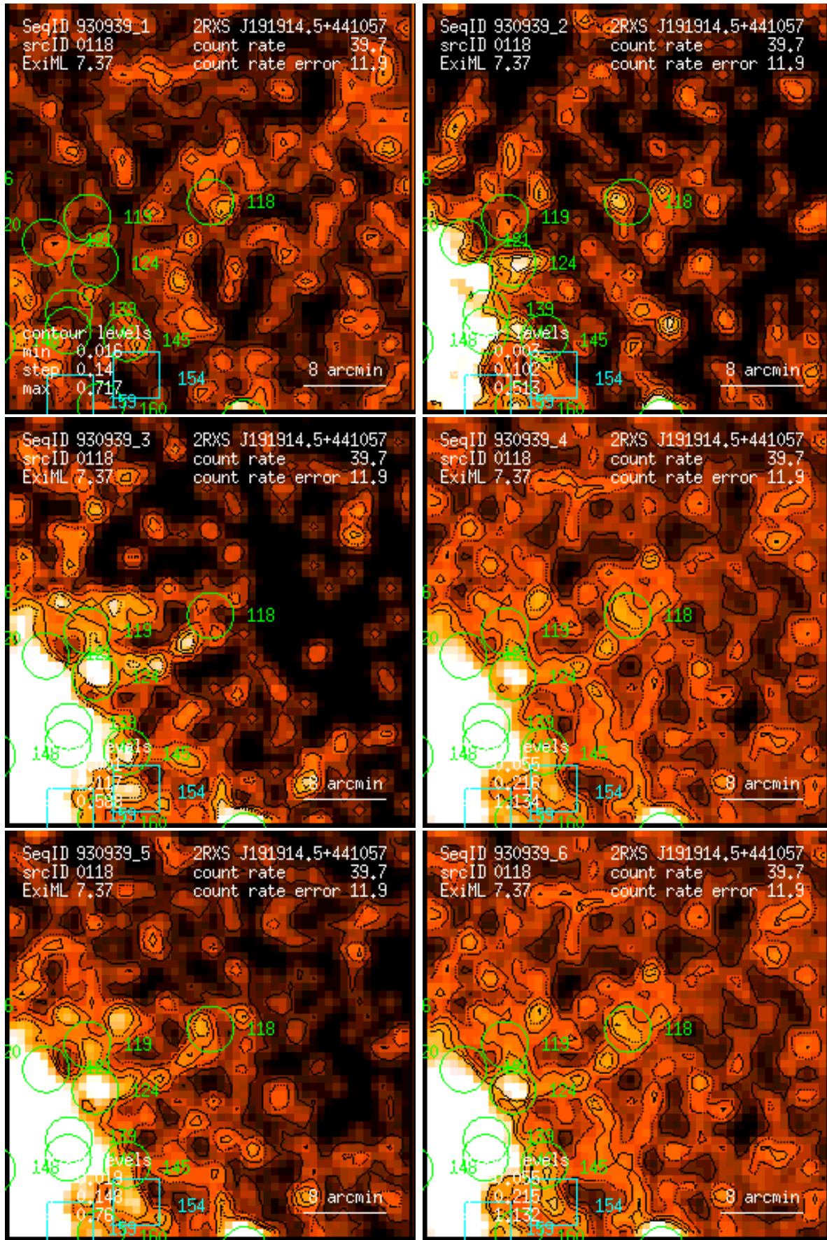
Figure 118: RASS 930939: detection 0118: band rate images, Gaussian filter: (1) PSPC channels 11 – 41, (2) 52 – 90, (3) 91 – 201, (4) 11 – 235, (5) 52 – 201, (6) 11 – 201. Broad band rates in counts/ks. Band rate contour levels in counts/ks/arcmin 2 .
