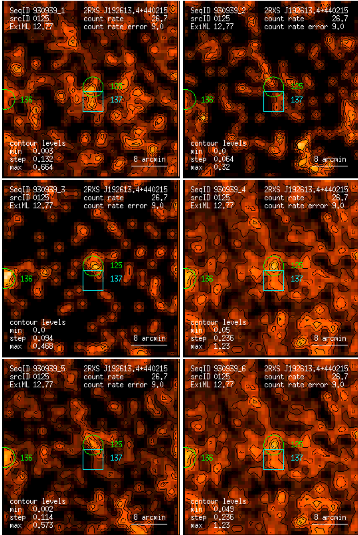
Figure 125: RASS 930939: detection 0125: band rate images, Gaussian filter: (1) PSPC channels 11 – 41, (2) 52 – 90, (3) 91 – 201, (4) 11 – 235, (5) 52 – 201, (6) 11 – 201. Broad band rates in counts/ks. Band rate contour levels in counts/ks/arcmin 2 .
