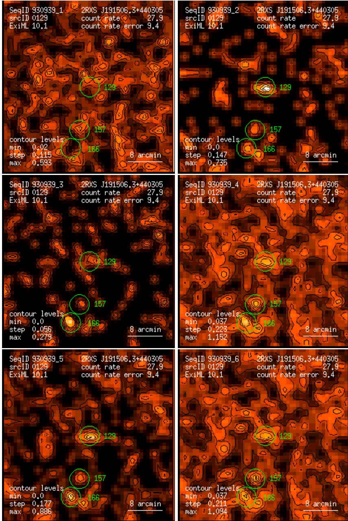
Figure 129: RASS 930939: detection 0129: band rate images, Gaussian filter: (1) PSPC channels 11 – 41, (2) 52 – 90, (3) 91 – 201, (4) 11 – 235, (5) 52 – 201, (6) 11 – 201. Broad band rates in counts/ks. Band rate contour levels in counts/ks/arcmin 2 .
