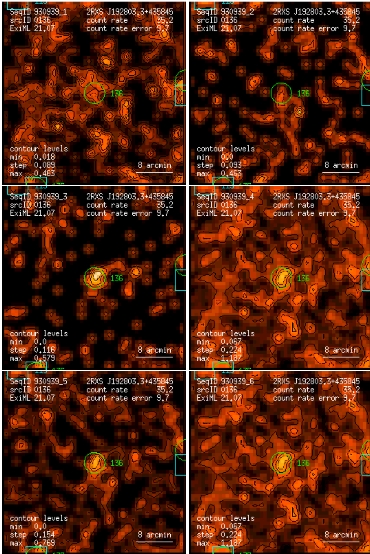
Figure 136: RASS 930939: detection 0136: band rate images, Gaussian filter: (1) PSPC channels 11 – 41, (2) 52 – 90, (3) 91 – 201, (4) 11 – 235, (5) 52 – 201, (6) 11 – 201. Broad band rates in counts/ks. Band rate contour levels in counts/ks/arcmin 2 .
