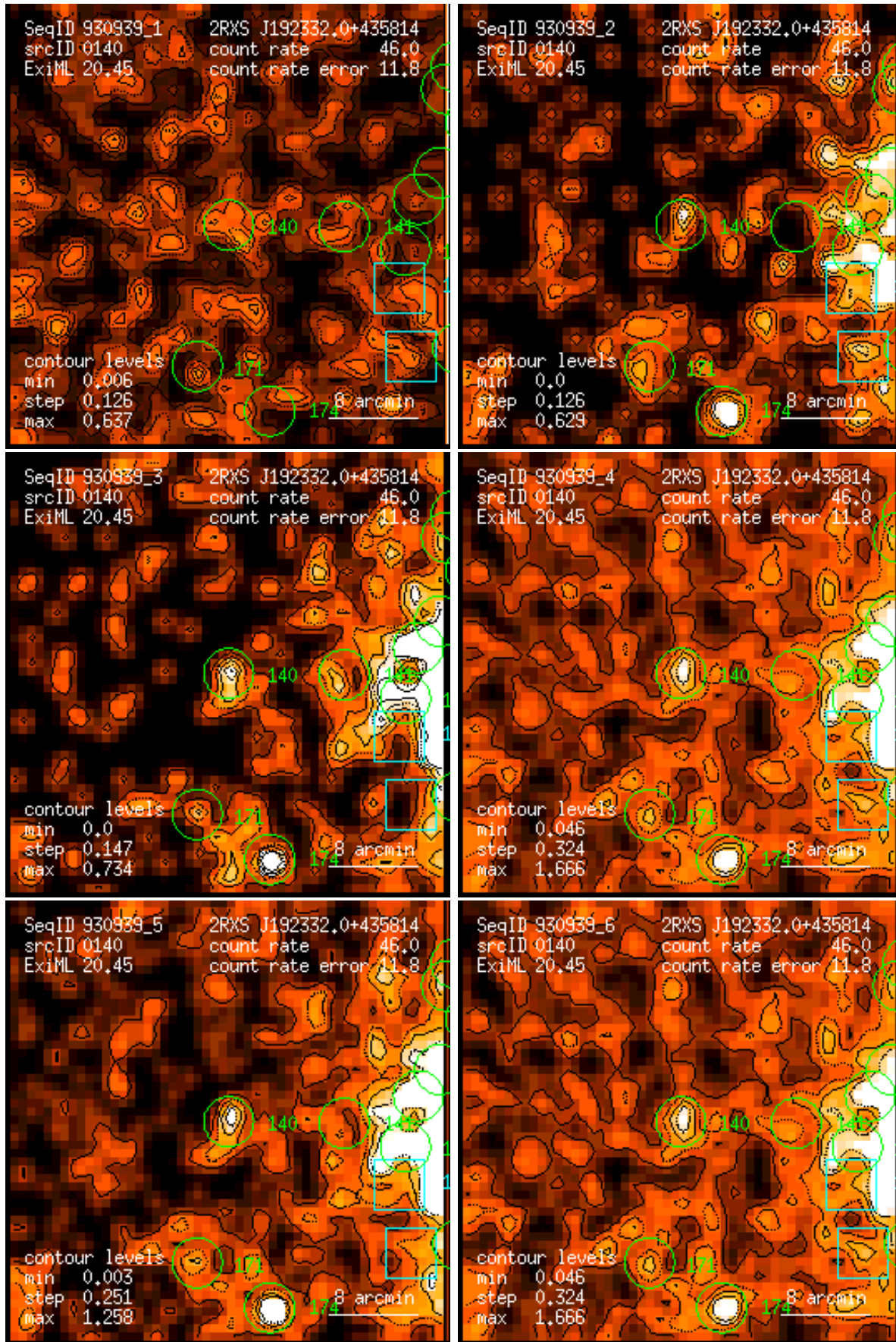
Figure 140: RASS 930939: detection 0140: band rate images, Gaussian filter: (1) PSPC channels 11 – 41, (2) 52 – 90, (3) 91 – 201, (4) 11 – 235, (5) 52 – 201, (6) 11 – 201. Broad band rates in counts/ks. Band rate contour levels in counts/ks/arcmin 2 .
