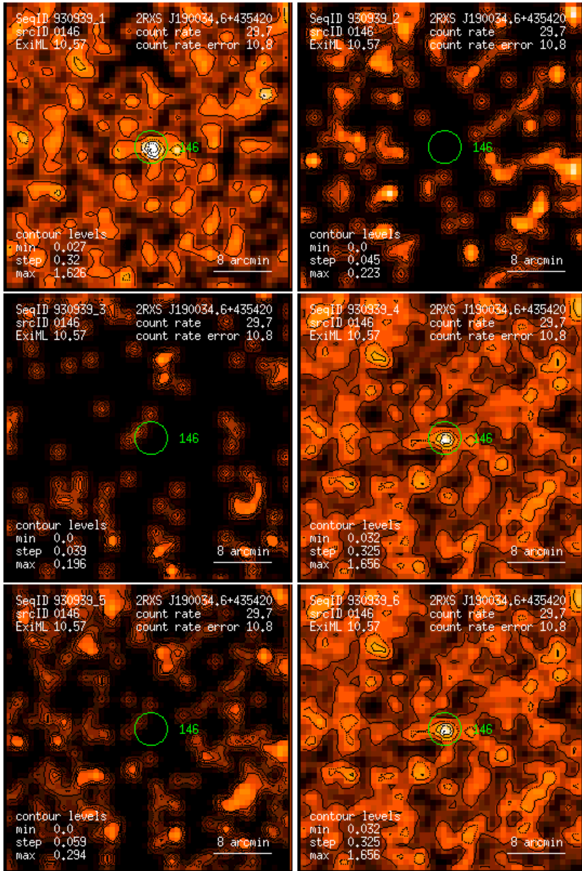
Figure 146: RASS 930939: detection 0146: band rate images, Gaussian filter: (1) PSPC channels 11 – 41, (2) 52 – 90, (3) 91 – 201, (4) 11 – 235, (5) 52 – 201, (6) 11 – 201. Broad band rates in counts/ks. Band rate contour levels in counts/ks/arcmin 2 .
