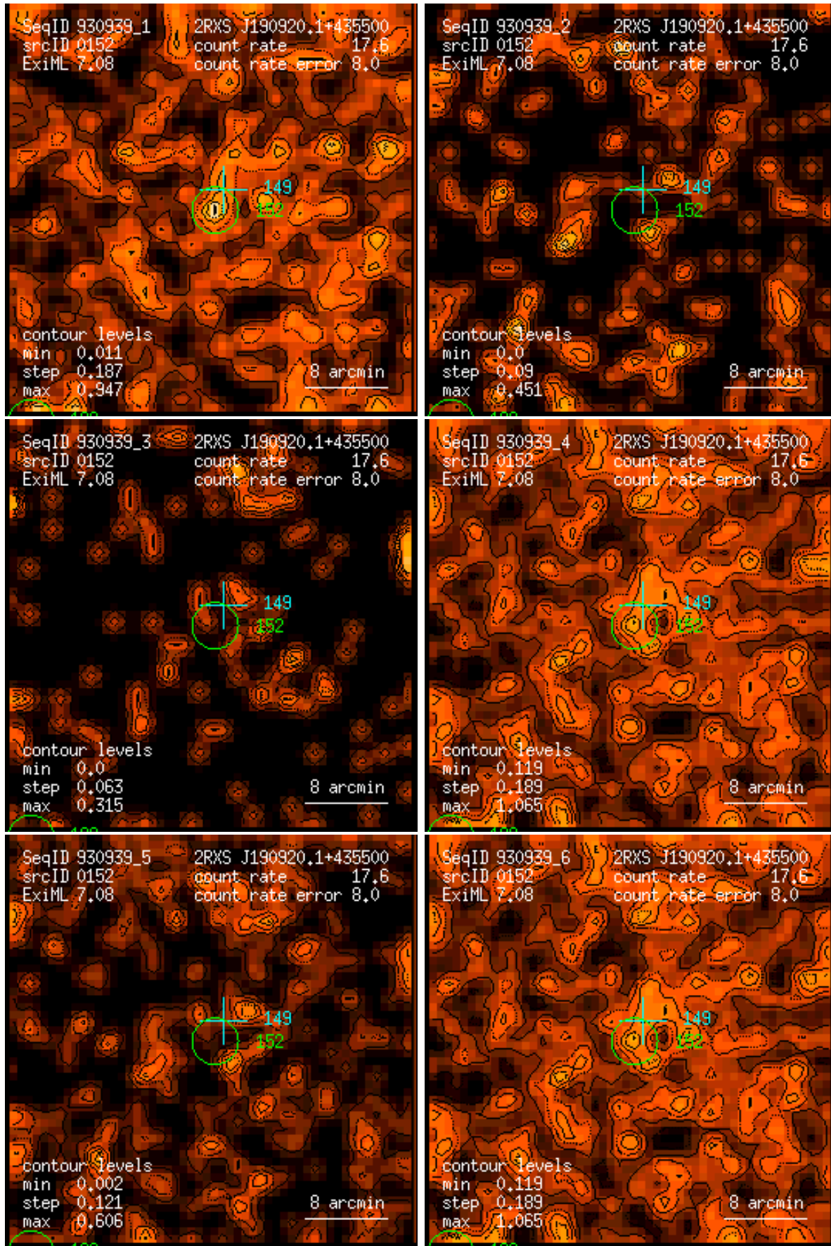
Figure 152: RASS 930939: detection 0152: band rate images, Gaussian filter: (1) PSPC channels 11 – 41, (2) 52 – 90, (3) 91 – 201, (4) 11 – 235, (5) 52 – 201, (6) 11 – 201. Broad band rates in counts/ks. Band rate contour levels in counts/ks/arcmin 2 .
