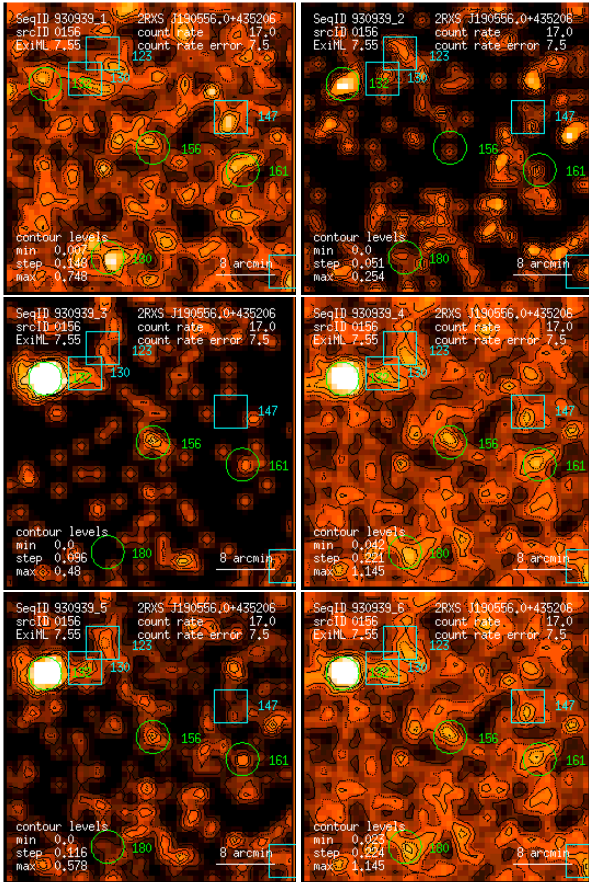
Figure 156: RASS 930939: detection 0156: band rate images, Gaussian filter: (1) PSPC channels 11 – 41, (2) 52 – 90, (3) 91 – 201, (4) 11 – 235, (5) 52 – 201, (6) 11 – 201. Broad band rates in counts/ks. Band rate contour levels in counts/ks/arcmin 2 .
