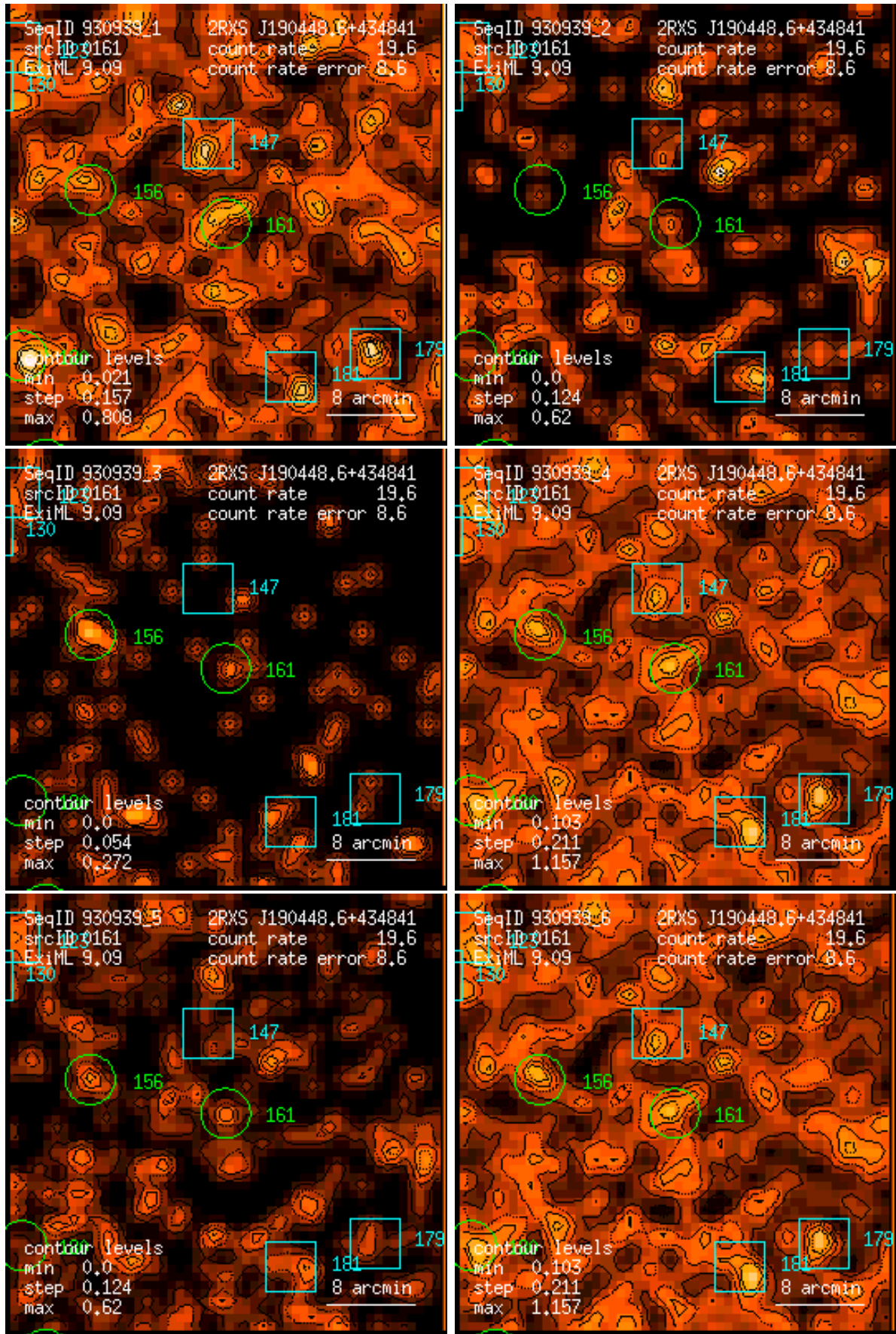
Figure 161: RASS 930939: detection 0161: band rate images, Gaussian filter: (1) PSPC channels 11 – 41, (2) 52 – 90, (3) 91 – 201, (4) 11 – 235, (5) 52 – 201, (6) 11 – 201. Broad band rates in counts/ks. Band rate contour levels in counts/ks/arcmin 2 .
