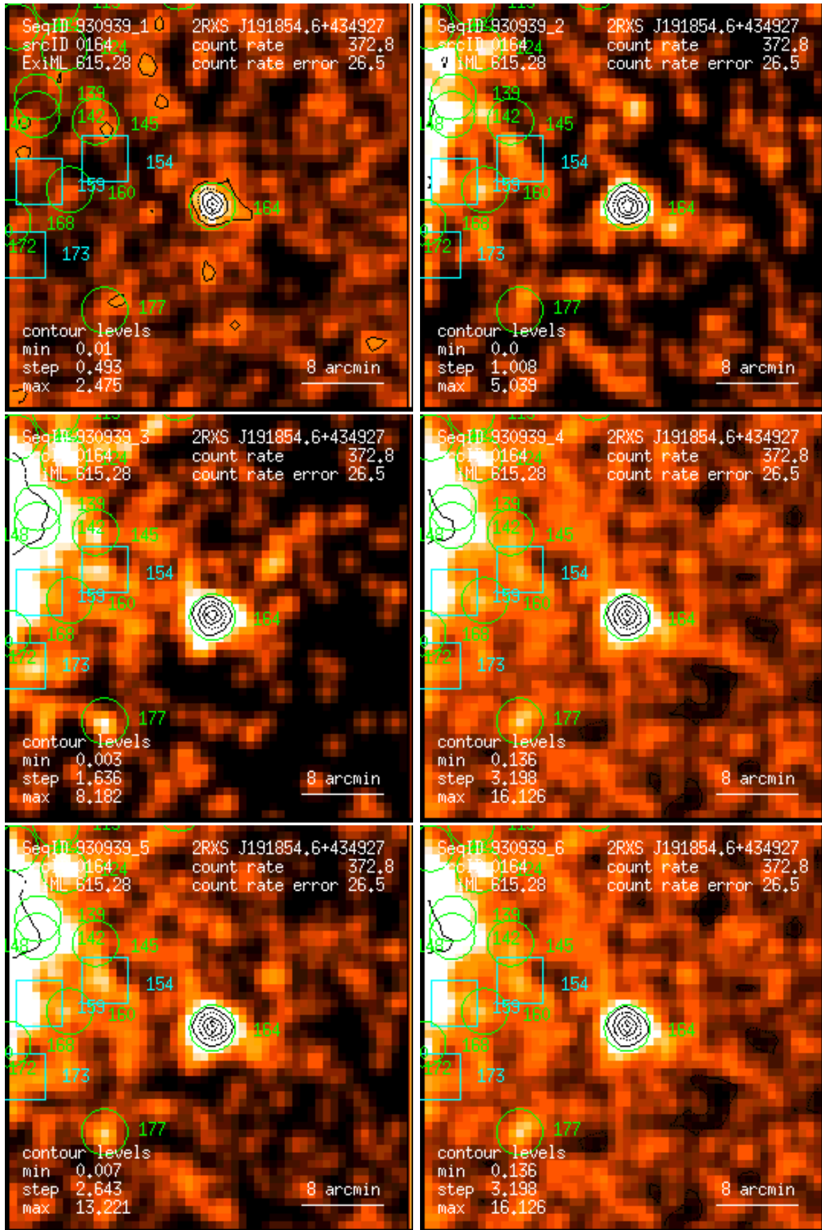
Figure 164: RASS 930939: detection 0164: band rate images, Gaussian filter: (1) PSPC channels 11 – 41, (2) 52 – 90, (3) 91 – 201, (4) 11 – 235, (5) 52 – 201, (6) 11 – 201. Broad band rates in counts/ks. Band rate contour levels in counts/ks/arcmin 2 .
