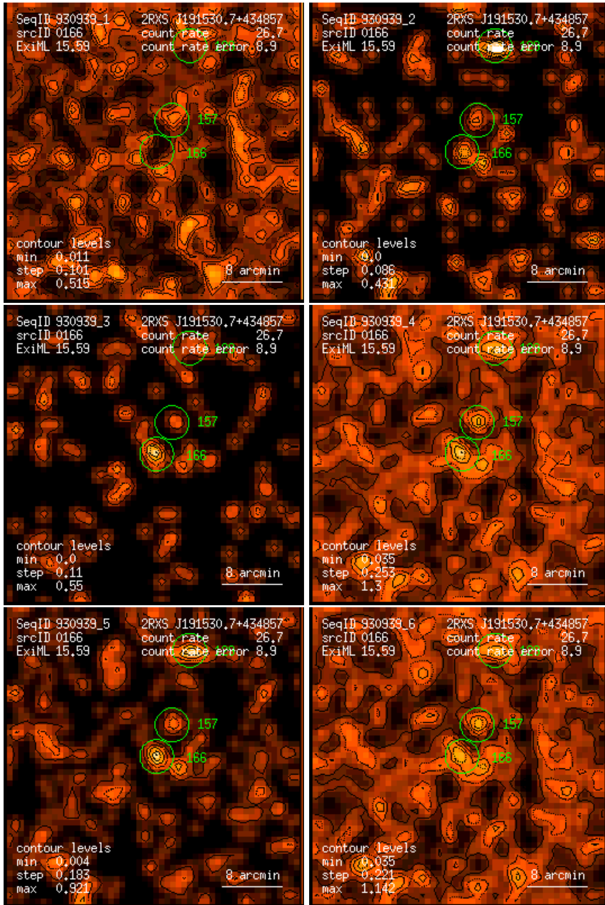
Figure 166: RASS 930939: detection 0166: band rate images, Gaussian filter: (1) PSPC channels 11 – 41, (2) 52 – 90, (3) 91 – 201, (4) 11 – 235, (5) 52 – 201, (6) 11 – 201. Broad band rates in counts/ks. Band rate contour levels in counts/ks/arcmin 2 .
