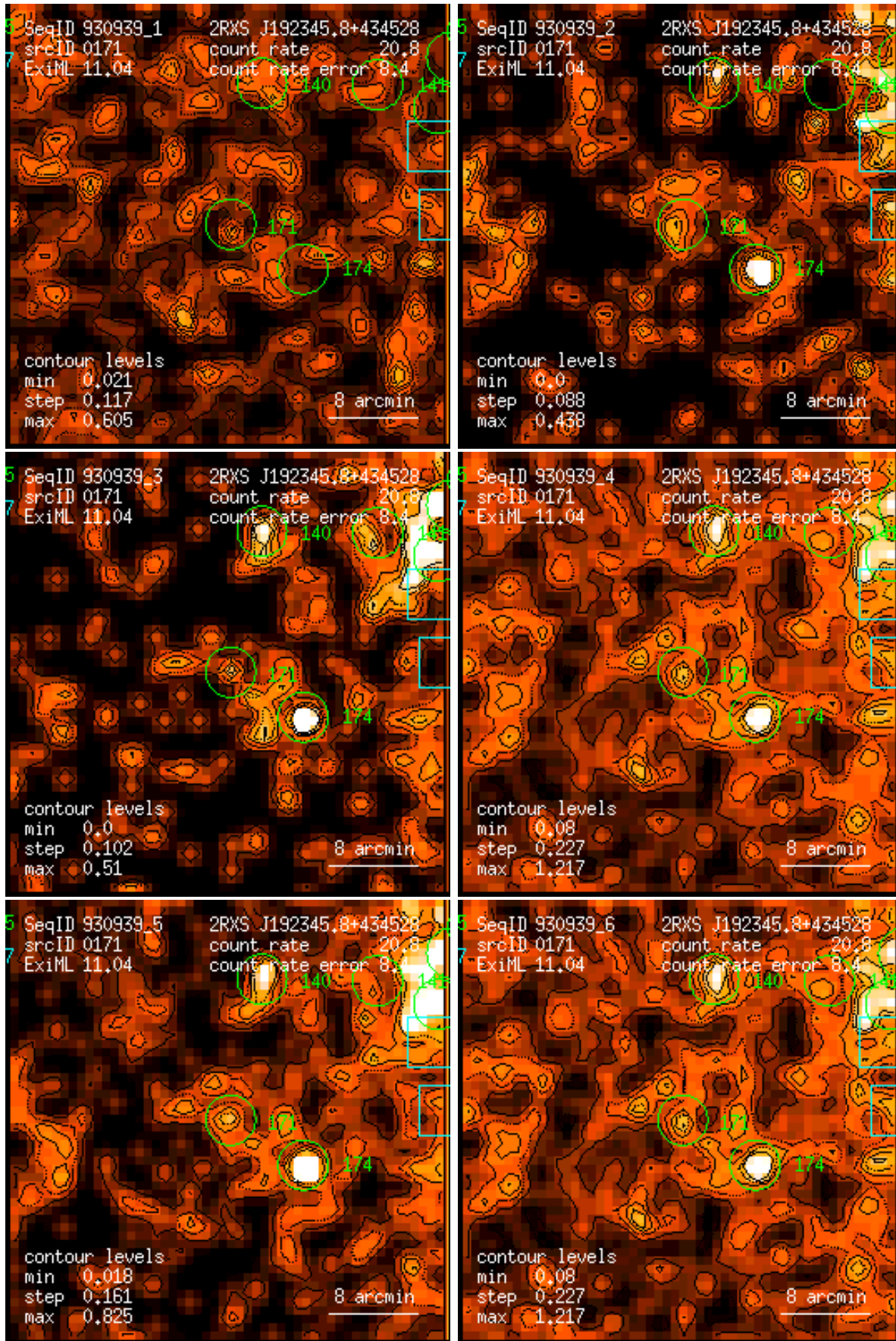
Figure 171: RASS 930939: detection 0171: band rate images, Gaussian filter: (1) PSPC channels 11 – 41, (2) 52 – 90, (3) 91 – 201, (4) 11 – 235, (5) 52 – 201, (6) 11 – 201. Broad band rates in counts/ks. Band rate contour levels in counts/ks/arcmin 2 .
