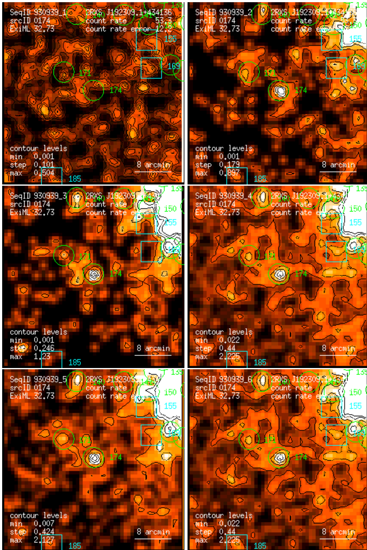
Figure 174: RASS 930939: detection 0174: band rate images, Gaussian filter: (1) PSPC channels 11 – 41, (2) 52 – 90, (3) 91 – 201, (4) 11 – 235, (5) 52 – 201, (6) 11 – 201. Broad band rates in counts/ks. Band rate contour levels in counts/ks/arcmin 2 .
