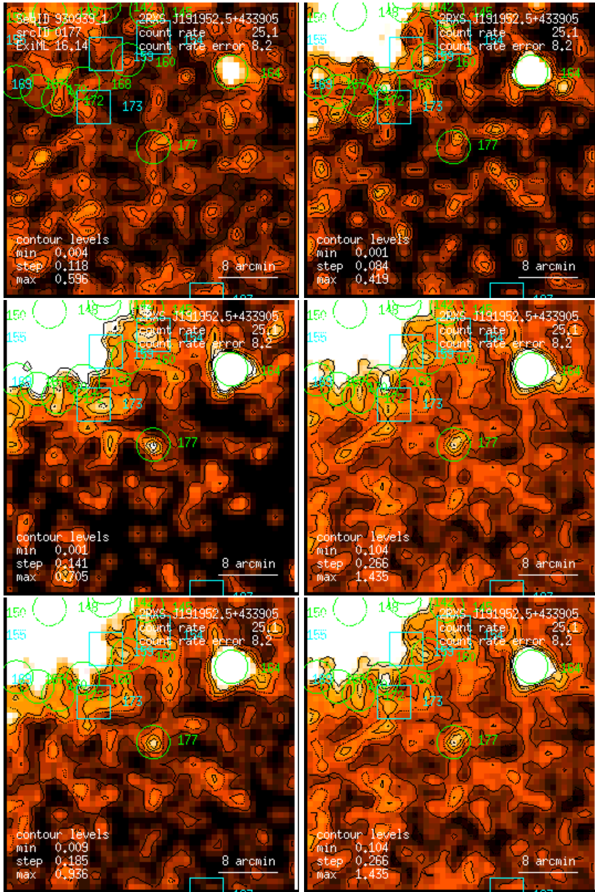
Figure 177: RASS 930939: detection 0177: band rate images, Gaussian filter: (1) PSPC channels 11 – 41, (2) 52 – 90, (3) 91 – 201, (4) 11 – 235, (5) 52 – 201, (6) 11 – 201. Broad band rates in counts/ks. Band rate contour levels in counts/ks/arcmin 2 .
