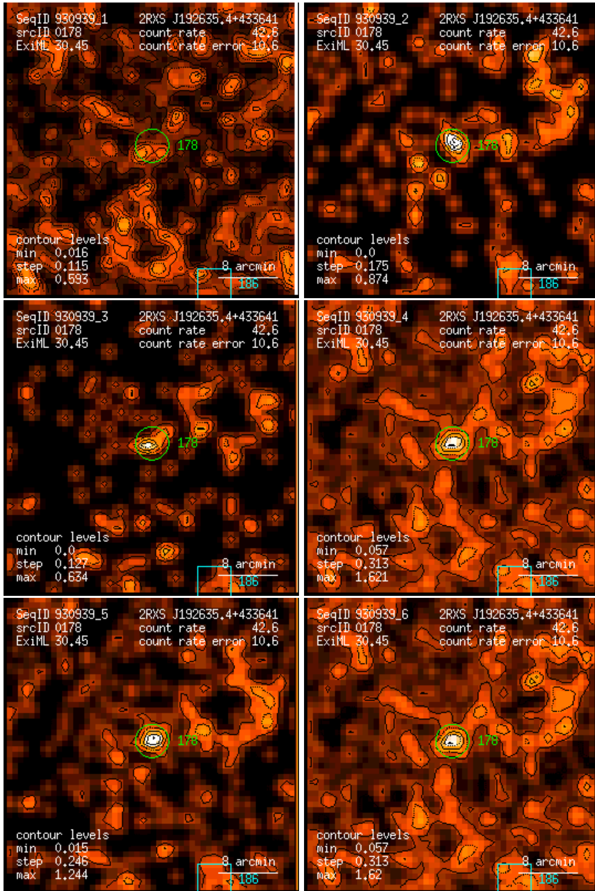
Figure 178: RASS 930939: detection 0178: band rate images, Gaussian filter: (1) PSPC channels 11 – 41, (2) 52 – 90, (3) 91 – 201, (4) 11 – 235, (5) 52 – 201, (6) 11 – 201. Broad band rates in counts/ks. Band rate contour levels in counts/ks/arcmin 2 .
