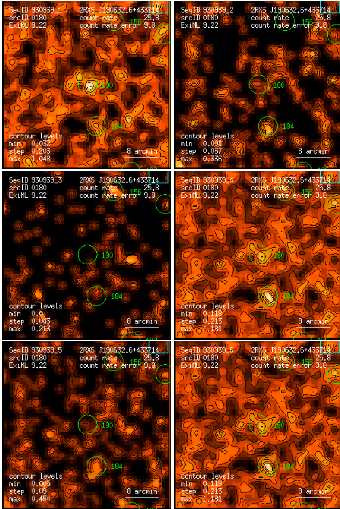
Figure 180: RASS 930939: detection 0180: band rate images, Gaussian filter: (1) PSPC channels 11 – 41, (2) 52 – 90, (3) 91 – 201, (4) 11 – 235, (5) 52 – 201, (6) 11 – 201. Broad band rates in counts/ks. Band rate contour levels in counts/ks/arcmin 2 .
