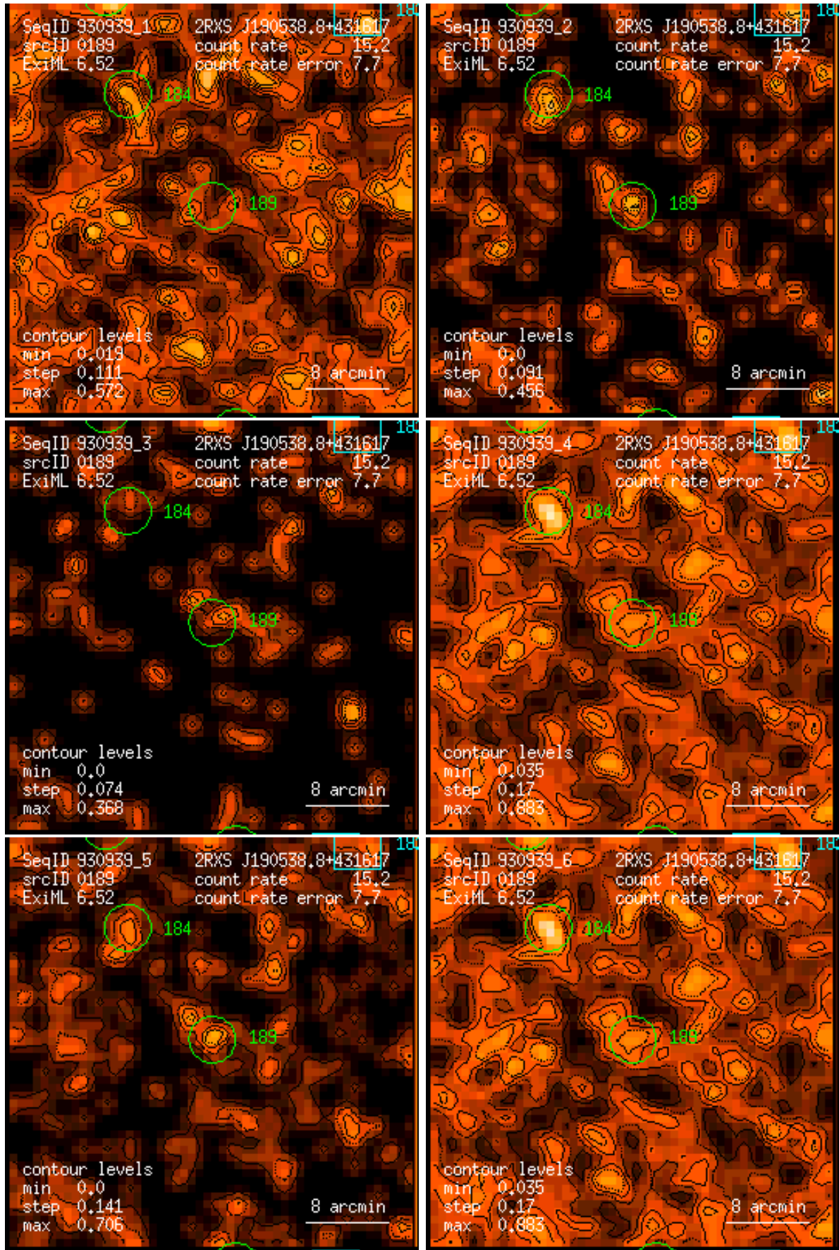
Figure 189: RASS 930939: detection 0189: band rate images, Gaussian filter: (1) PSPC channels 11 – 41, (2) 52 – 90, (3) 91 – 201, (4) 11 – 235, (5) 52 – 201, (6) 11 – 201. Broad band rates in counts/ks. Band rate contour levels in counts/ks/arcmin 2 .
