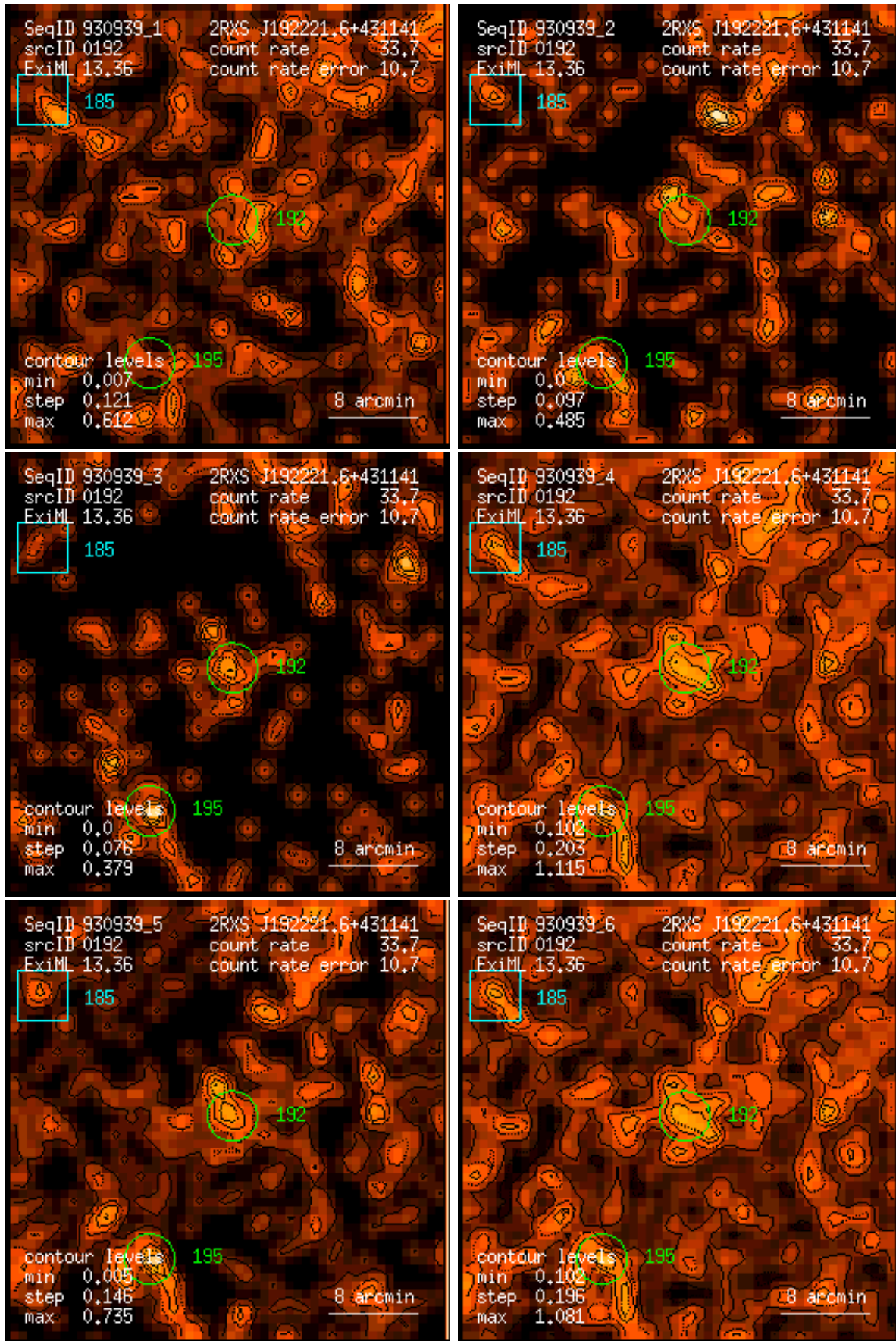
Figure 192: RASS 930939: detection 0192: band rate images, Gaussian filter: (1) PSPC channels 11 – 41, (2) 52 – 90, (3) 91 – 201, (4) 11 – 235, (5) 52 – 201, (6) 11 – 201. Broad band rates in counts/ks. Band rate contour levels in counts/ks/arcmin 2 .
