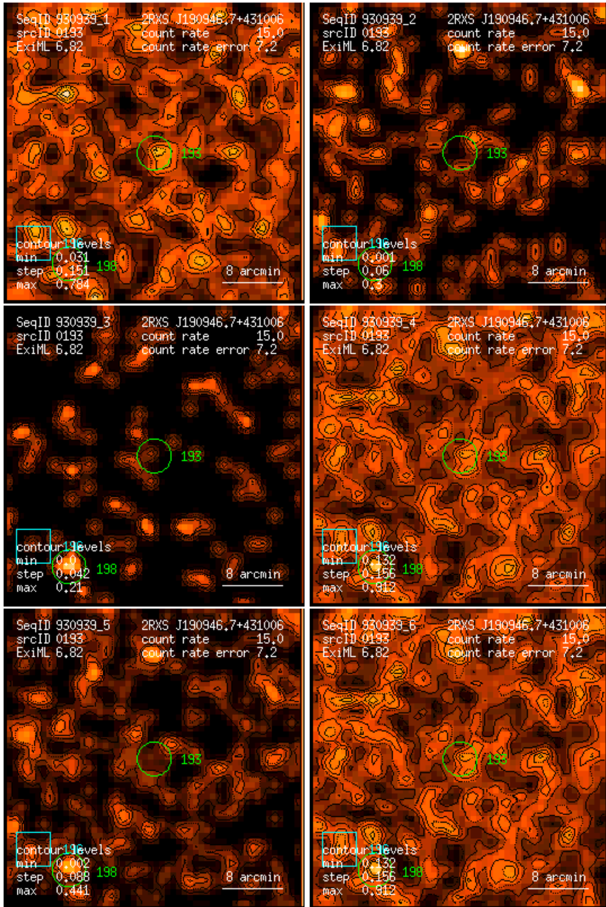
Figure 193: RASS 930939: detection 0193: band rate images, Gaussian filter: (1) PSPC channels 11 – 41, (2) 52 – 90, (3) 91 – 201, (4) 11 – 235, (5) 52 – 201, (6) 11 – 201. Broad band rates in counts/ks. Band rate contour levels in counts/ks/arcmin 2 .
