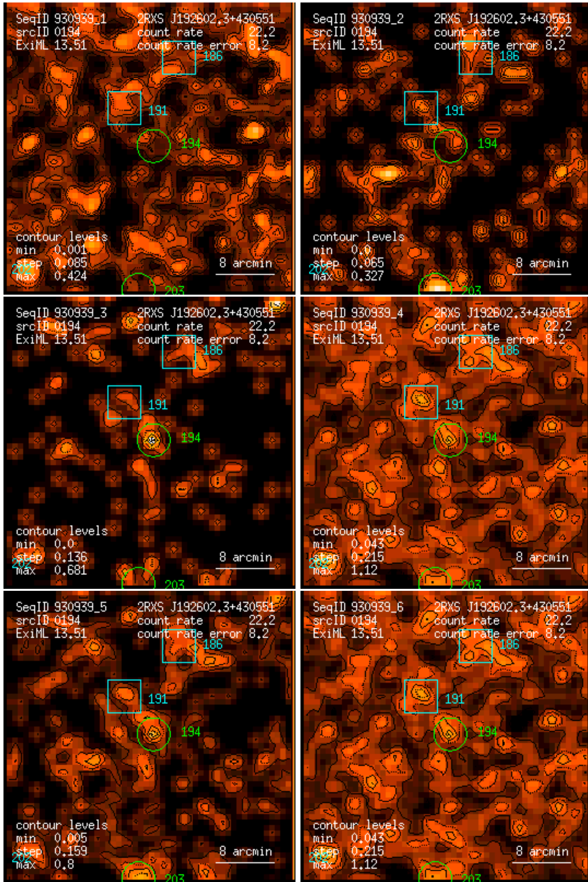
Figure 194: RASS 930939: detection 0194: band rate images, Gaussian filter: (1) PSPC channels 11 – 41, (2) 52 – 90, (3) 91 – 201, (4) 11 – 235, (5) 52 – 201, (6) 11 – 201. Broad band rates in counts/ks. Band rate contour levels in counts/ks/arcmin 2 .
