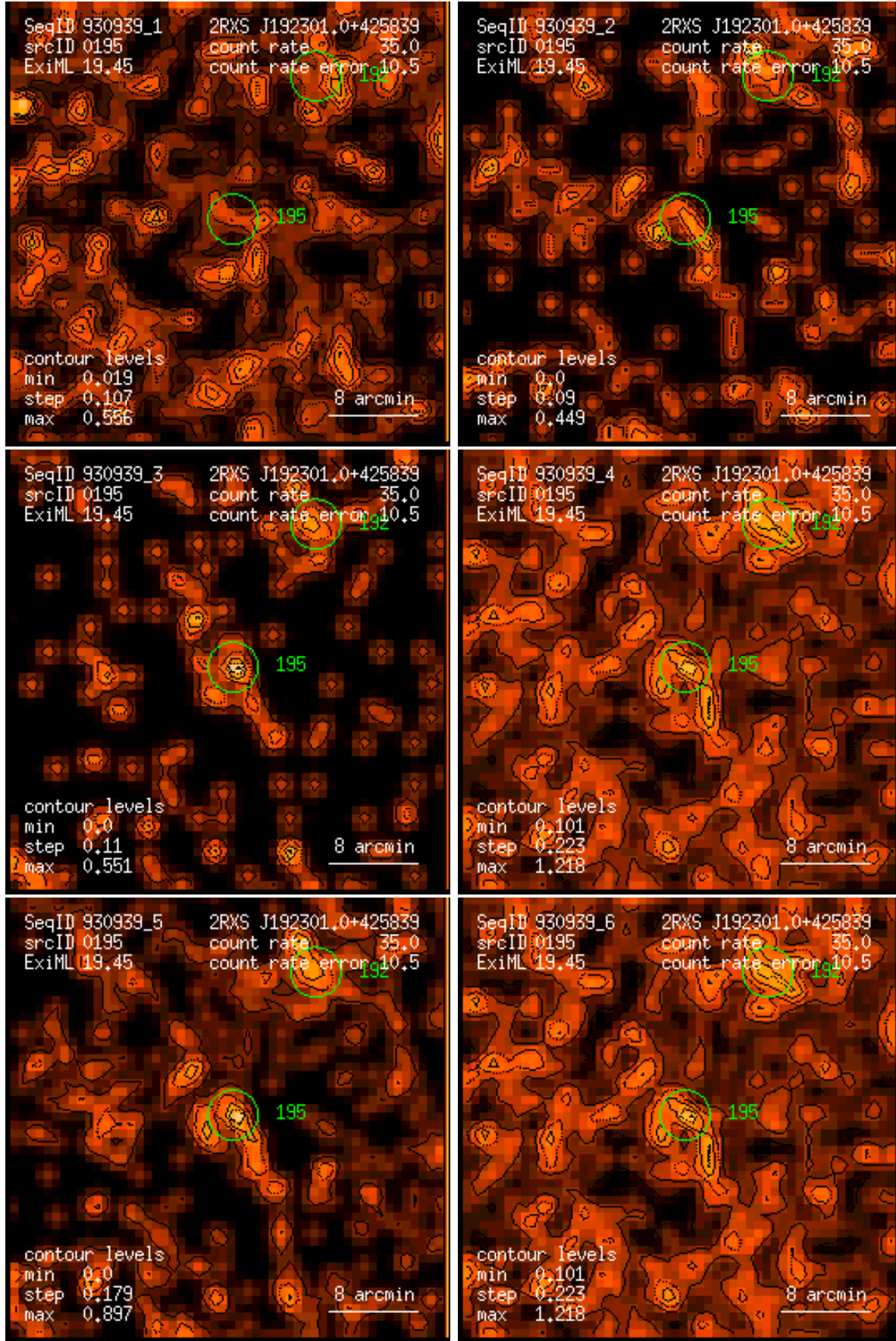
Figure 195: RASS 930939: detection 0195: band rate images, Gaussian filter: (1) PSPC channels 11 – 41, (2) 52 – 90, (3) 91 – 201, (4) 11 – 235, (5) 52 – 201, (6) 11 – 201. Broad band rates in counts/ks. Band rate contour levels in counts/ks/arcmin 2 .
