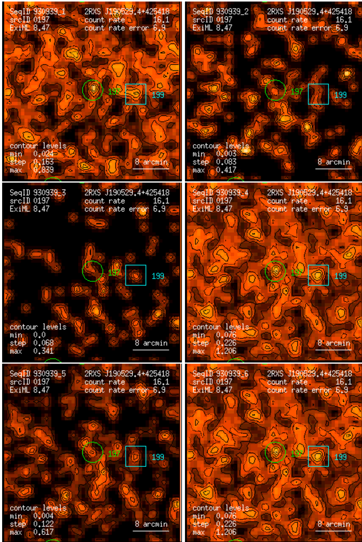
Figure 197: RASS 930939: detection 0197: band rate images, Gaussian filter: (1) PSPC channels 11 – 41, (2) 52 – 90, (3) 91 – 201, (4) 11 – 235, (5) 52 – 201, (6) 11 – 201. Broad band rates in counts/ks. Band rate contour levels in counts/ks/arcmin 2 .
