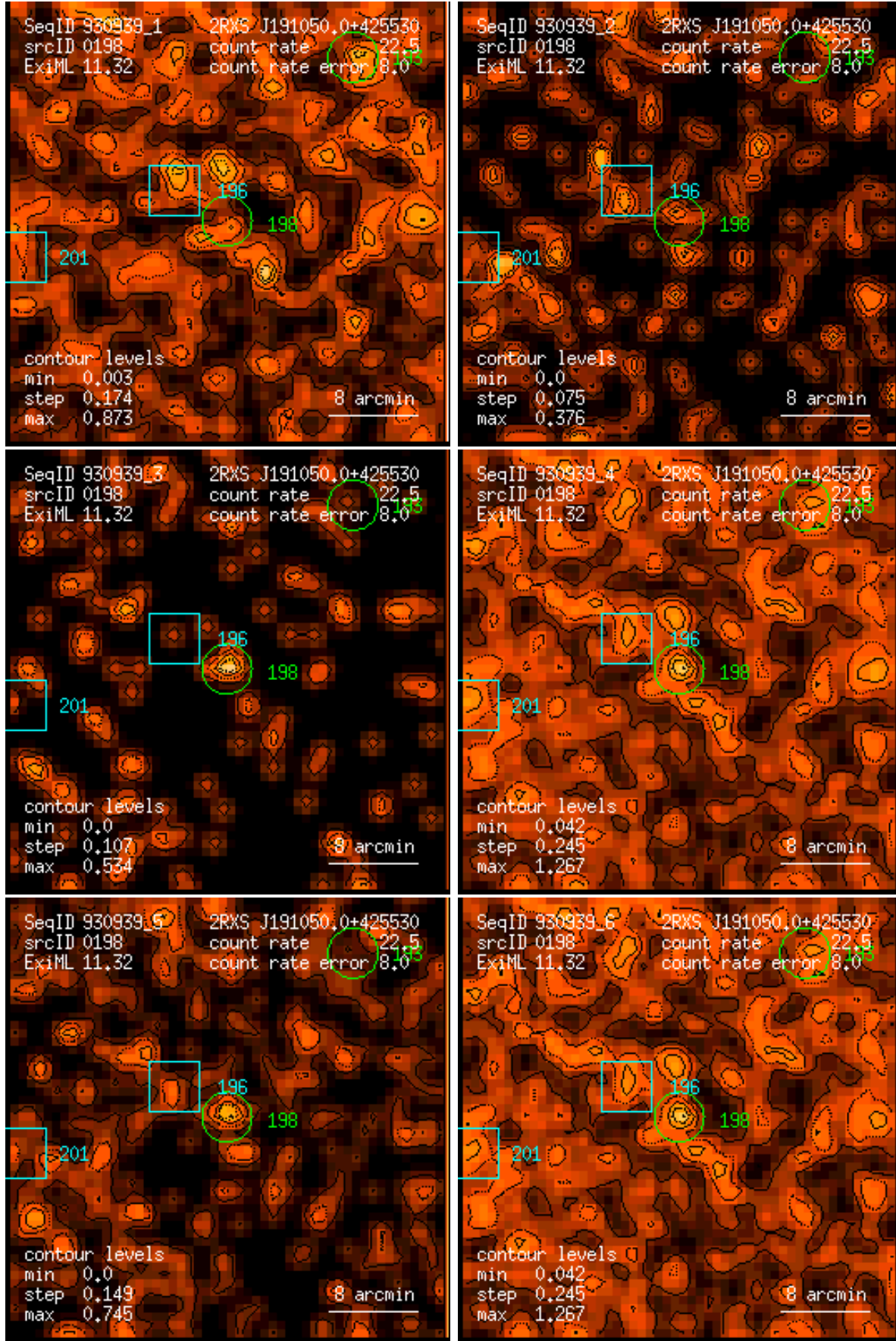
Figure 198: RASS 930939: detection 0198: band rate images, Gaussian filter: (1) PSPC channels 11 – 41, (2) 52 – 90, (3) 91 – 201, (4) 11 – 235, (5) 52 – 201, (6) 11 – 201. Broad band rates in counts/ks. Band rate contour levels in counts/ks/arcmin 2 .
