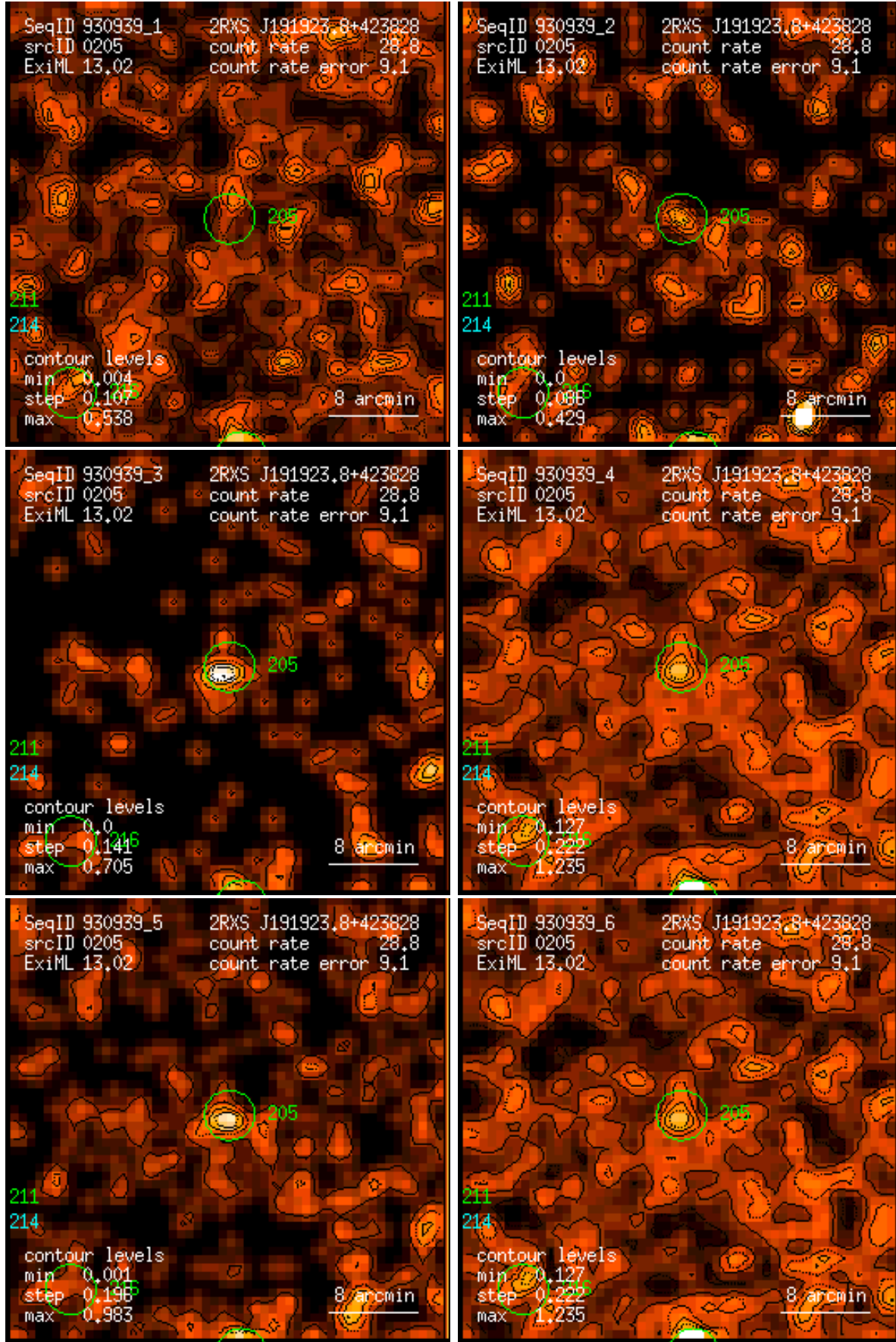
Figure 205: RASS 930939: detection 0205: band rate images, Gaussian filter: (1) PSPC channels 11 – 41, (2) 52 – 90, (3) 91 – 201, (4) 11 – 235, (5) 52 – 201, (6) 11 – 201. Broad band rates in counts/ks. Band rate contour levels in counts/ks/arcmin 2 .
