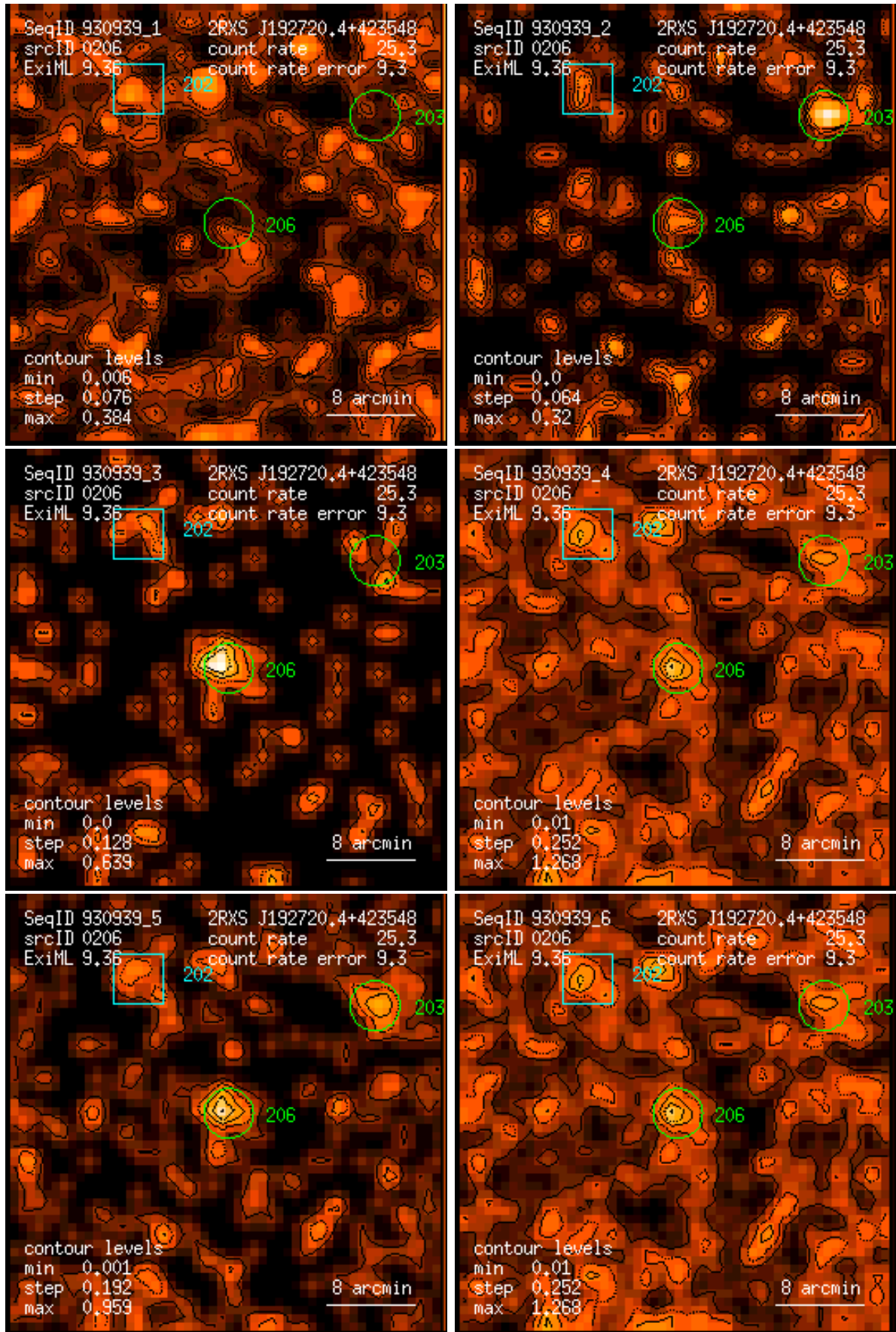
Figure 206: RASS 930939: detection 0206: band rate images, Gaussian filter: (1) PSPC channels 11 – 41, (2) 52 – 90, (3) 91 – 201, (4) 11 – 235, (5) 52 – 201, (6) 11 – 201. Broad band rates in counts/ks. Band rate contour levels in counts/ks/arcmin 2 .
