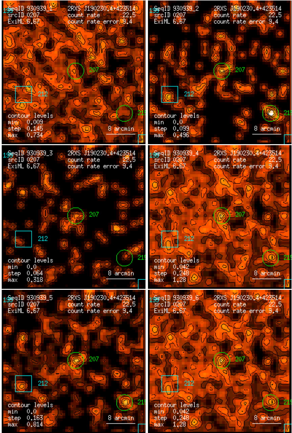
Figure 207: RASS 930939: detection 0207: band rate images, Gaussian filter: (1) PSPC channels 11 – 41, (2) 52 – 90, (3) 91 – 201, (4) 11 – 235, (5) 52 – 201, (6) 11 – 201. Broad band rates in counts/ks. Band rate contour levels in counts/ks/arcmin 2 .
