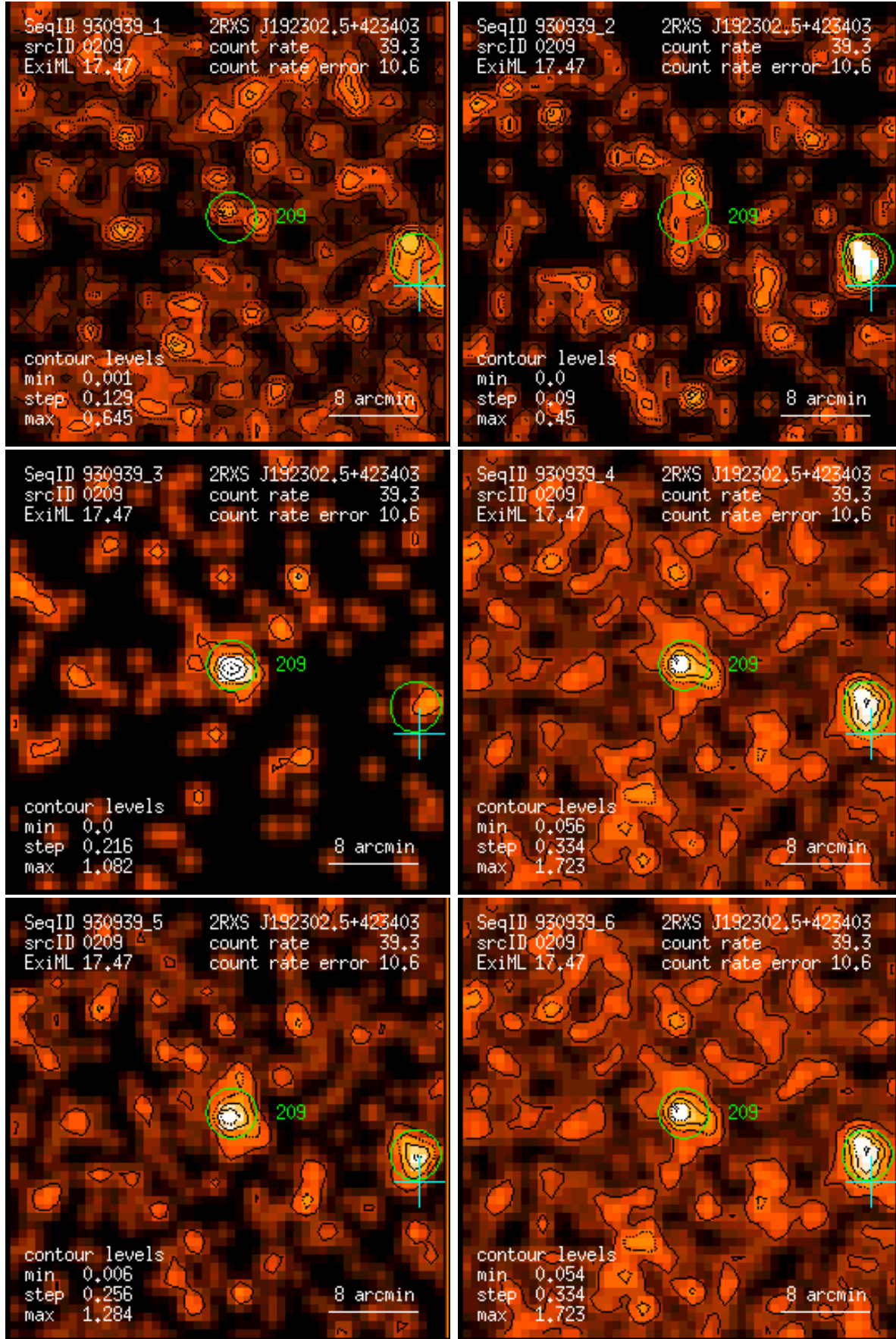
Figure 209: RASS 930939: detection 0209: band rate images, Gaussian filter: (1) PSPC channels 11 – 41, (2) 52 – 90, (3) 91 – 201, (4) 11 – 235, (5) 52 – 201, (6) 11 – 201. Broad band rates in counts/ks. Band rate contour levels in counts/ks/arcmin 2 .
