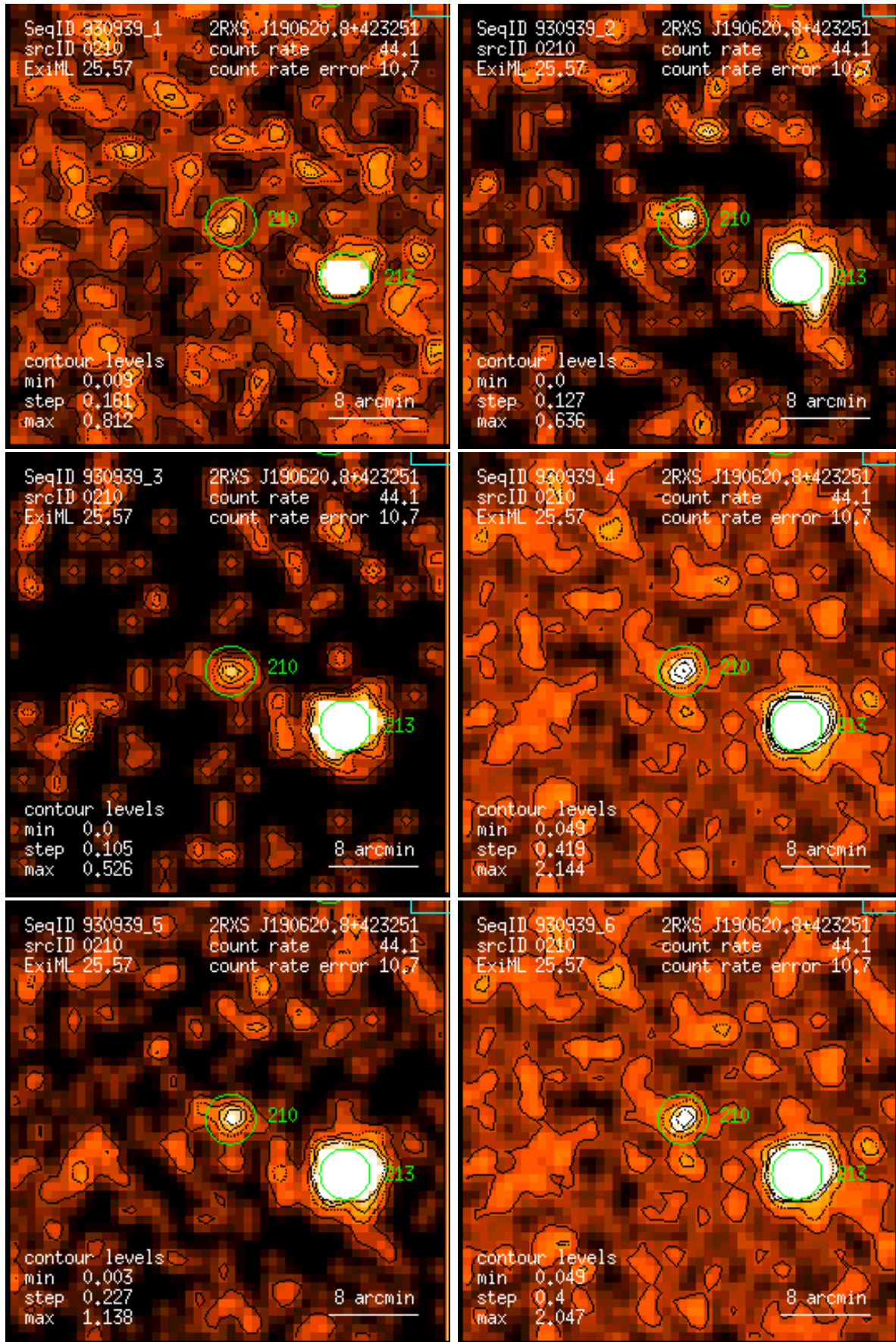
Figure 210: RASS 930939: detection 0210: band rate images, Gaussian filter: (1) PSPC channels 11 – 41, (2) 52 – 90, (3) 91 – 201, (4) 11 – 235, (5) 52 – 201, (6) 11 – 201. Broad band rates in counts/ks. Band rate contour levels in counts/ks/arcmin 2 .
