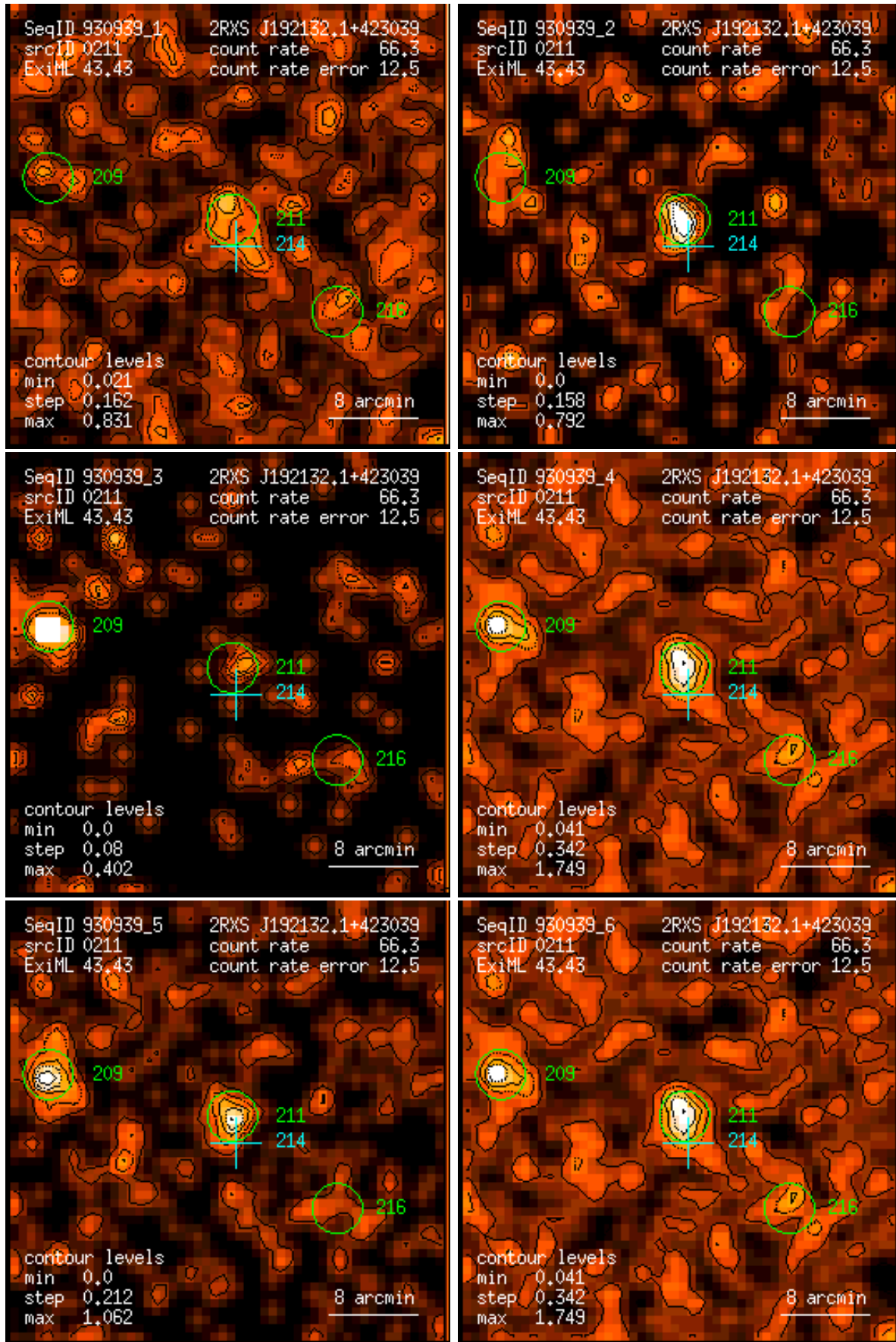
Figure 211: RASS 930939: detection 0211: band rate images, Gaussian filter: (1) PSPC channels 11 – 41, (2) 52 – 90, (3) 91 – 201, (4) 11 – 235, (5) 52 – 201, (6) 11 – 201. Broad band rates in counts/ks. Band rate contour levels in counts/ks/arcmin 2 .
