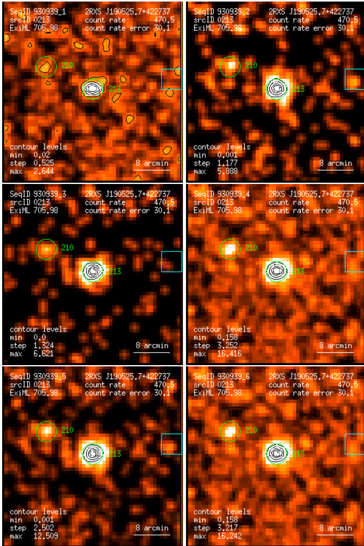
Figure 213: RASS 930939: detection 0213: band rate images, Gaussian filter: (1) PSPC channels 11 – 41, (2) 52 – 90, (3) 91 – 201, (4) 11 – 235, (5) 52 – 201, (6) 11 – 201. Broad band rates in counts/ks. Band rate contour levels in counts/ks/arcmin 2 .
