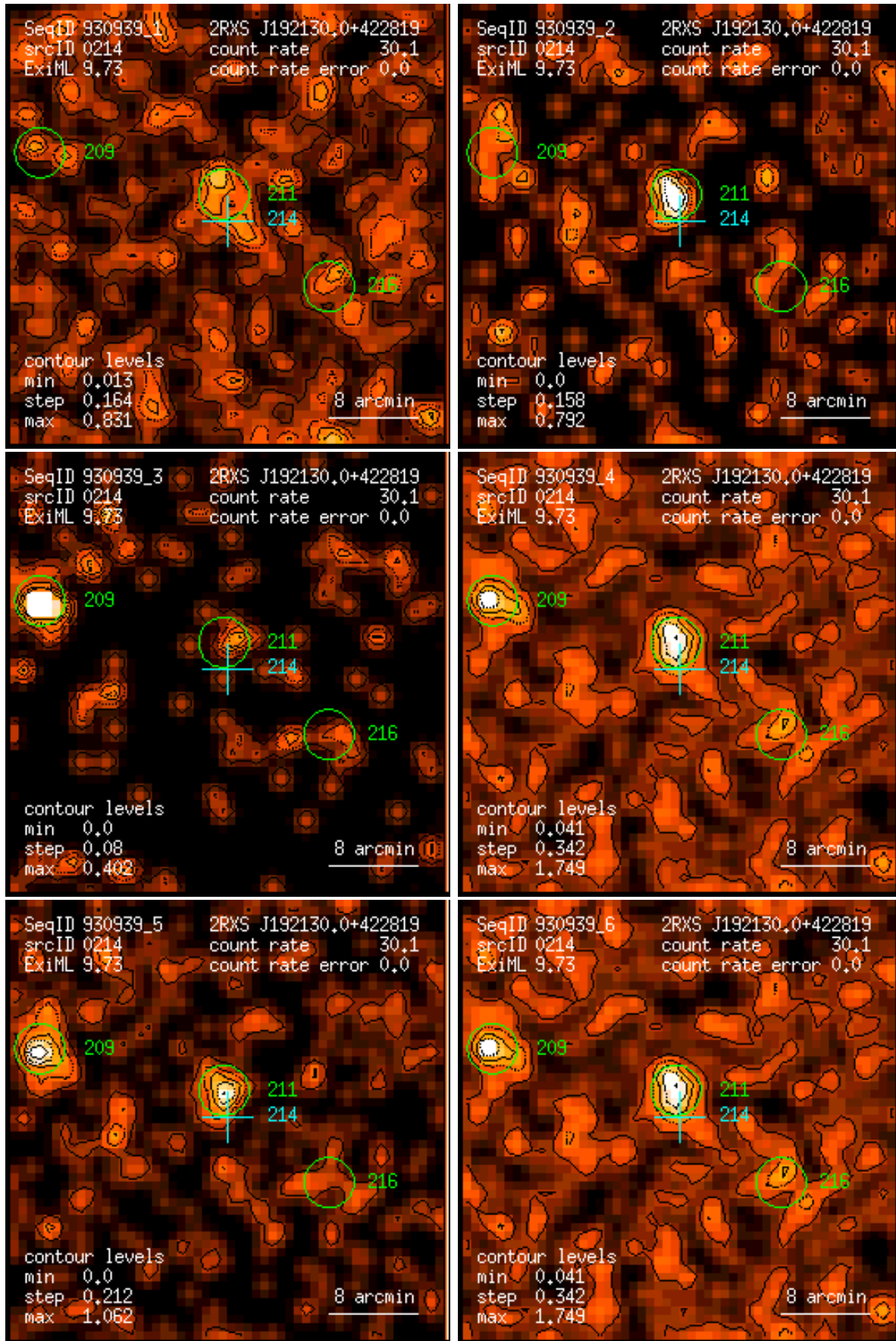
Figure 214: RASS 930939: detection 0214: band rate images, Gaussian filter: (1) PSPC channels 11 – 41, (2) 52 – 90, (3) 91 – 201, (4) 11 – 235, (5) 52 – 201, (6) 11 – 201. Broad band rates in counts/ks. Band rate contour levels in counts/ks/arcmin 2 .
