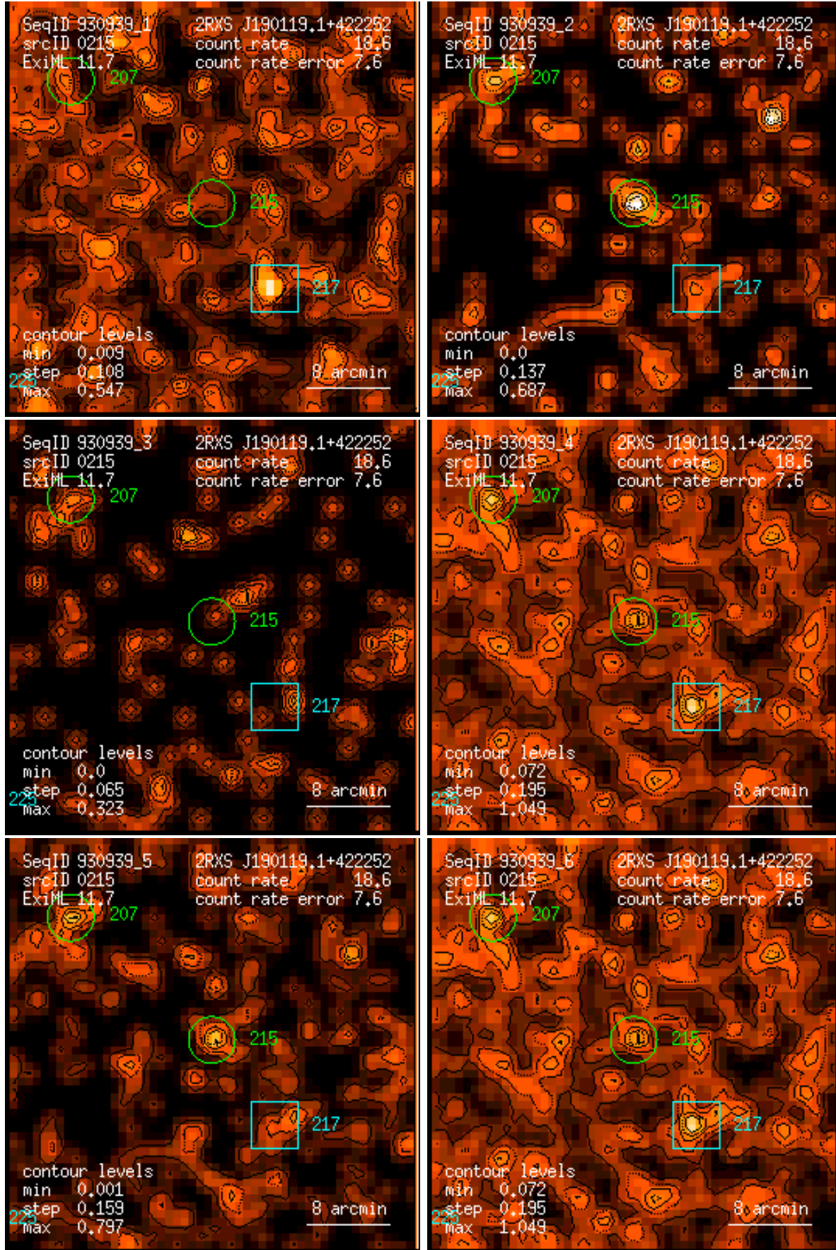
Figure 215: RASS 930939: detection 0215: band rate images, Gaussian filter: (1) PSPC channels 11 – 41, (2) 52 – 90, (3) 91 – 201, (4) 11 – 235, (5) 52 – 201, (6) 11 – 201. Broad band rates in counts/ks. Band rate contour levels in counts/ks/arcmin 2 .
