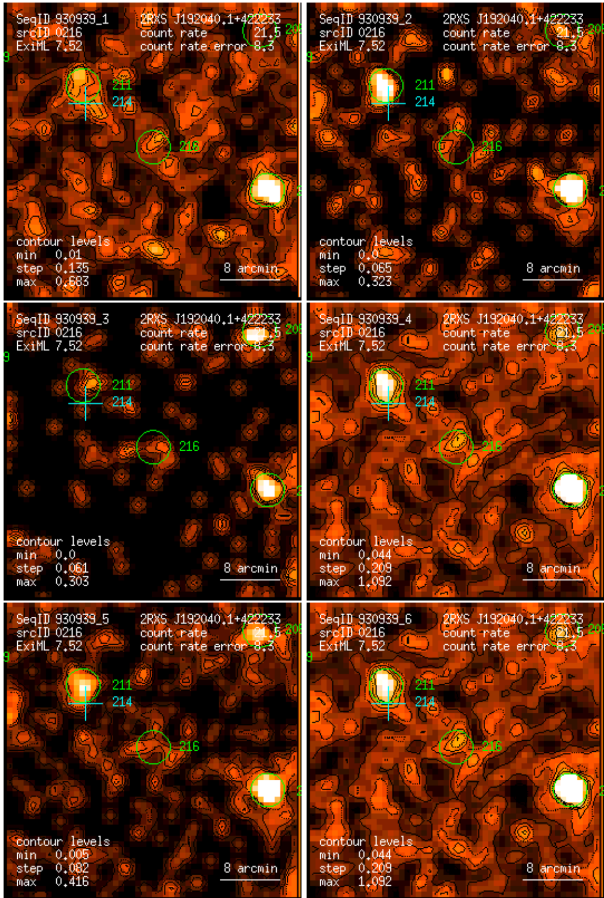
Figure 216: RASS 930939: detection 0216: band rate images, Gaussian filter: (1) PSPC channels 11 – 41, (2) 52 – 90, (3) 91 – 201, (4) 11 – 235, (5) 52 – 201, (6) 11 – 201. Broad band rates in counts/ks. Band rate contour levels in counts/ks/arcmin 2 .
