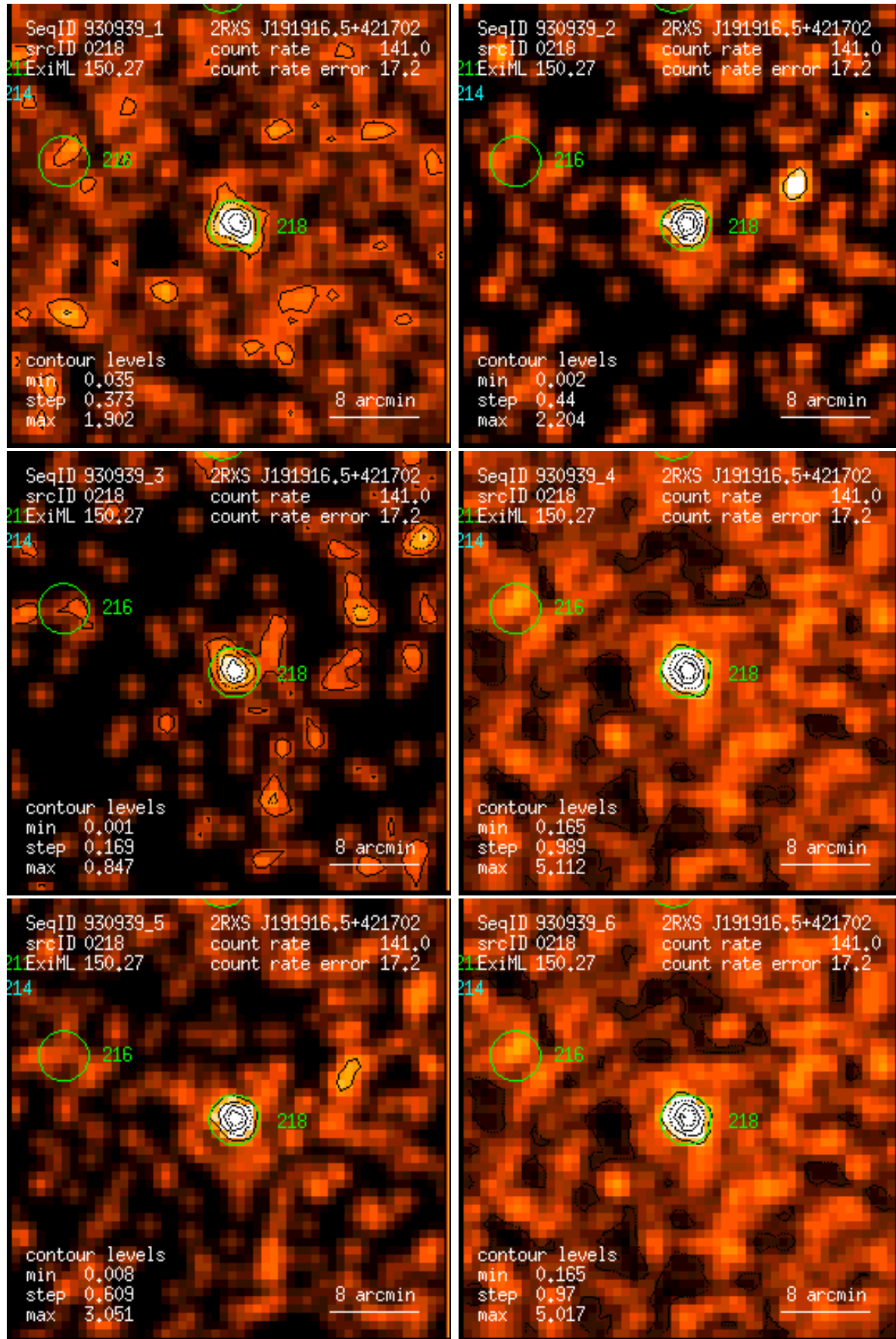
Figure 218: RASS 930939: detection 0218: band rate images, Gaussian filter: (1) PSPC channels 11 – 41, (2) 52 – 90, (3) 91 – 201, (4) 11 – 235, (5) 52 – 201, (6) 11 – 201. Broad band rates in counts/ks. Band rate contour levels in counts/ks/arcmin 2 .
