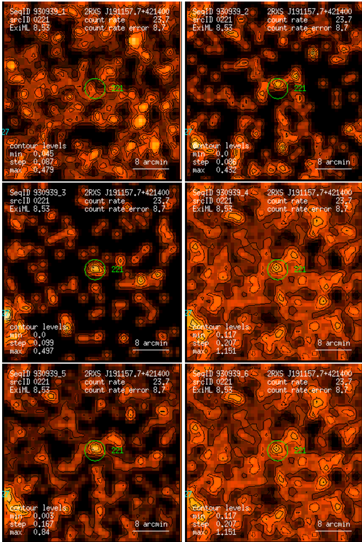
Figure 221: RASS 930939: detection 0221: band rate images, Gaussian filter: (1) PSPC channels 11 – 41, (2) 52 – 90, (3) 91 – 201, (4) 11 – 235, (5) 52 – 201, (6) 11 – 201. Broad band rates in counts/ks. Band rate contour levels in counts/ks/arcmin 2 .
