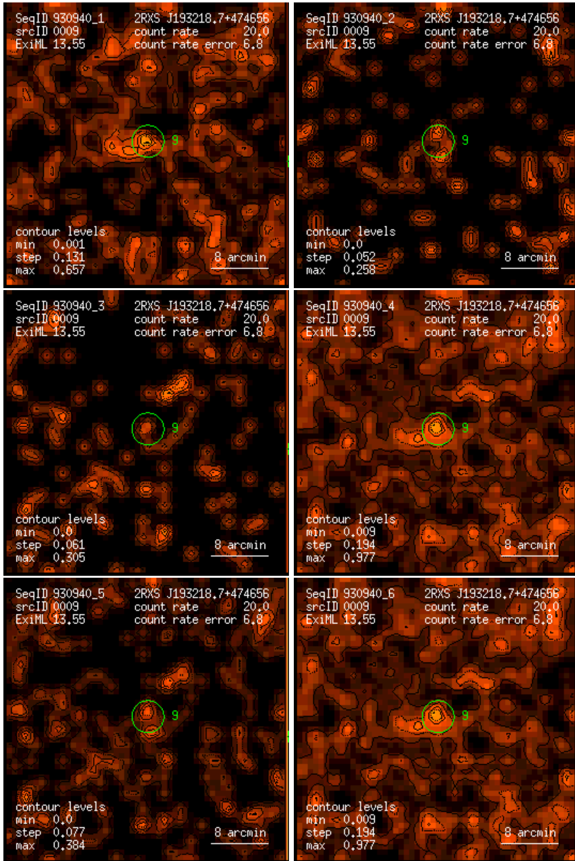
Figure 9: RASS 930940: detection 0009: band rate images, Gaussian filter: (1) PSPC channels 11 – 41, (2) 52 – 90, (3) 91 – 201, (4) 11 – 235, (5) 52 – 201, (6) 11 – 201. Broad band rates in counts/ks. Band rate contour levels in counts/ks/arcmin 2 .
